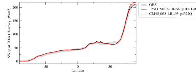
rsutcszone
