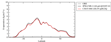
evazon
