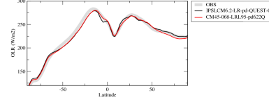
rlutzone
