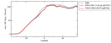
rsahzone
