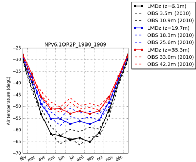
tempDC-NPv6.1OR2P_1980_1989
