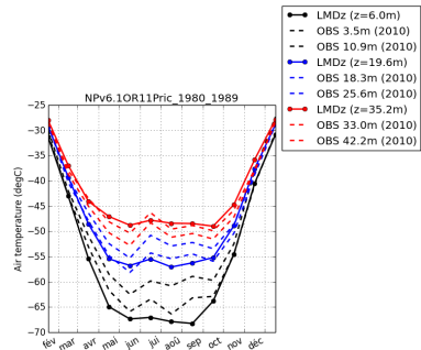
tempDC-NPv6.1OR11Pric_1980_1989
