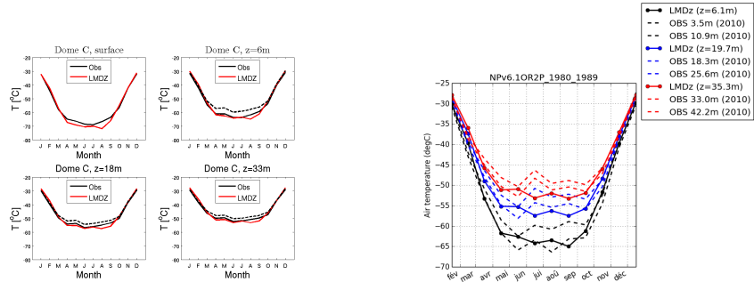
temp_DC_NPv6.1OR2P_1980_1989
