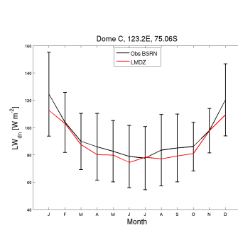
LWdnSFC_DC_NPv6.1OR11P_1980_1989
