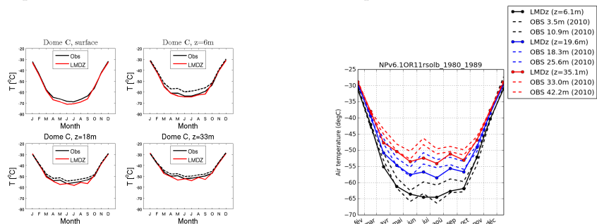
temp_DC_NPv6.1OR11rsolb_1980_1989
