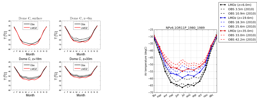
temp_DC_NPv6.1OR11P_1980_1989
