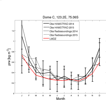
prw_DC_NPv6.1OR11rsolb_1980_1989
