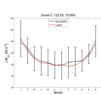
LWdnSFC_DC_NPv6.1OR2P_1980_1989
