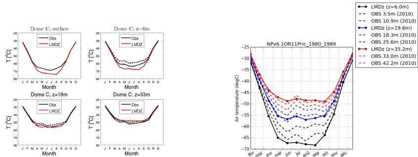
temp_DC_NPv6.1OR11Pric_1980_1989
