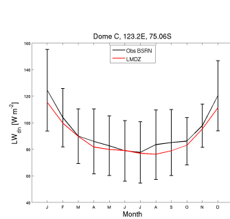
LWdnSFC_DC_NPv6.1OR11Pric_1980_1989
