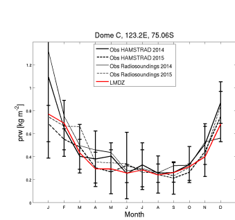
prw_DC_NPv6.1OR2P_1980_1989
