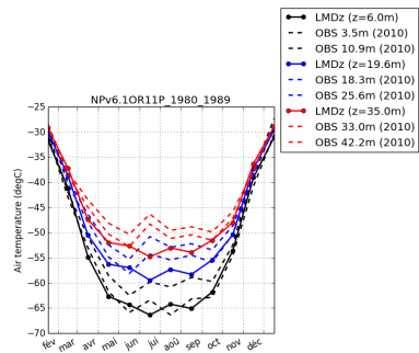
tempDC-NPv6.1OR11P_1980_1989
