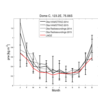
prw_DC_NPv6.1OR11P_1980_1989
