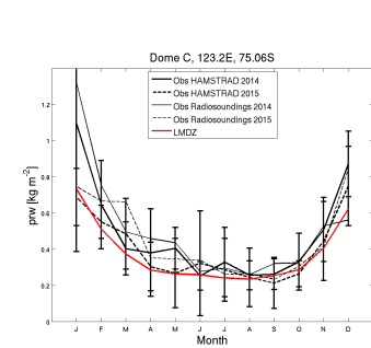
prw_DC_NPv6.1OR11Pric_1980_1989
