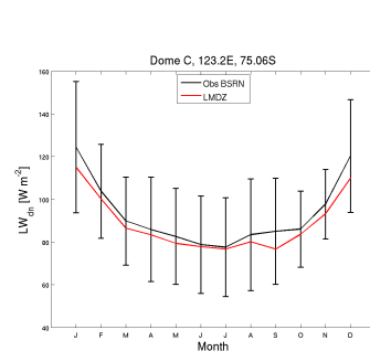
LWdnSFC_DC_NPv6.1OR11rsolb_1980_1989
