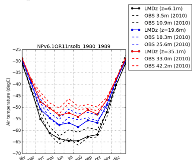
tempDC-NPv6.1OR11rsolb_1980_1989
