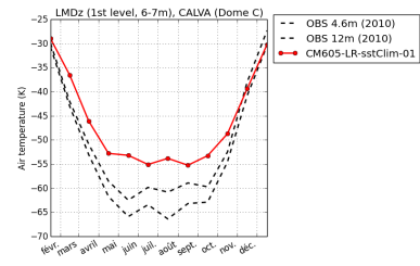
tempDC-CM605-LR-sstClim-01
