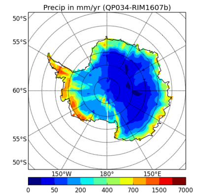
precipSH-QP034-RIM1607b
