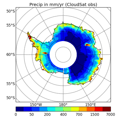
precipSH-OBS
