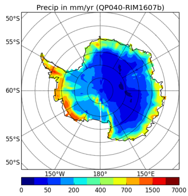
precipSH-QP040-RIM1607b
