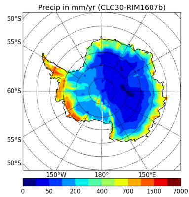
precipSH-CLC30-RIM1607b
