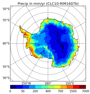
precipSH-CLC10-RIM1607b
