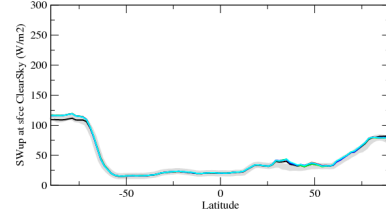
rsuscszon
