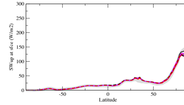
rsuszcn
