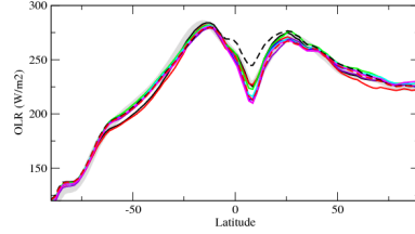
rlutzon
