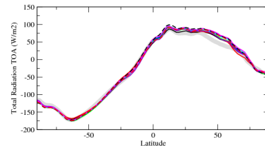
rttzcn
