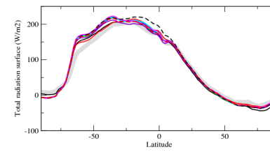
rtzone
