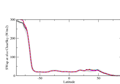
rsuscszone
