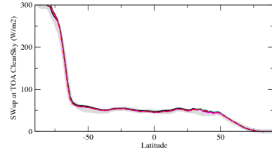
rsutcszone
