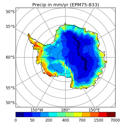
precipSH-EPM75-833
