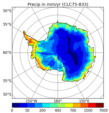
precipSH-CLC75-833
