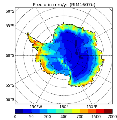
precipSH-RIM1607b
