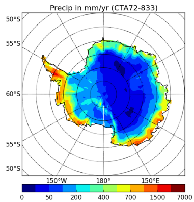
precipSH-CTA72-833
