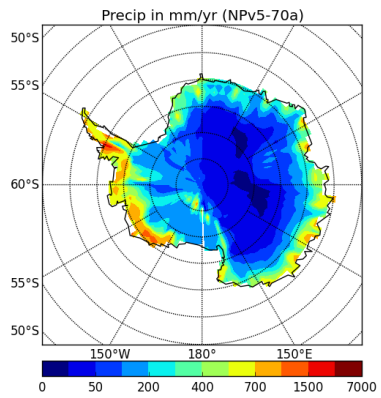
precipSH-NPv5-70a
