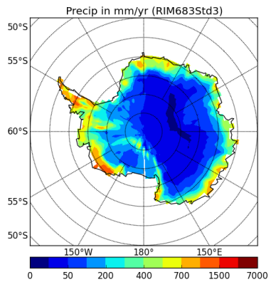
precipSH-RIM683Std3
