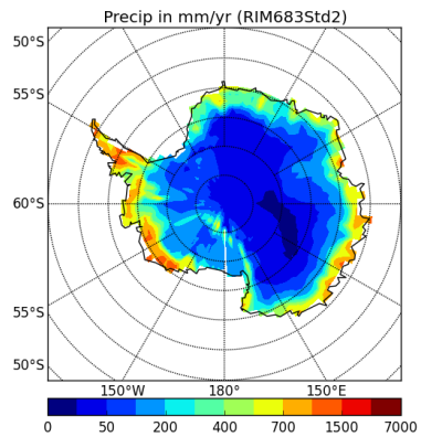
precipSH-RIM683Std2
