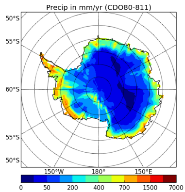
precipSH-CDO80-811
