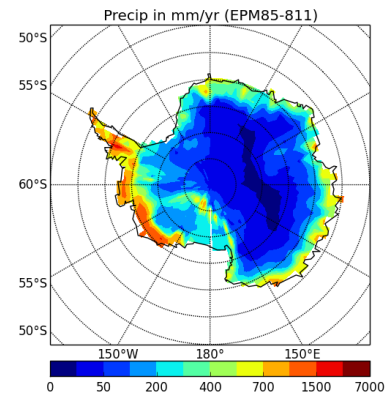
precipSH-EPM85-811
