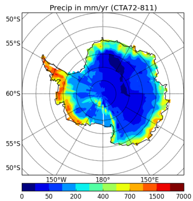
precipSH-CTA72-811
