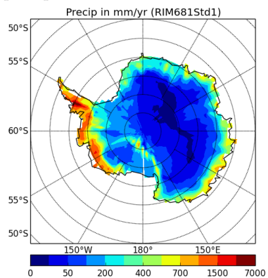
precipSH-RIM681Std1
