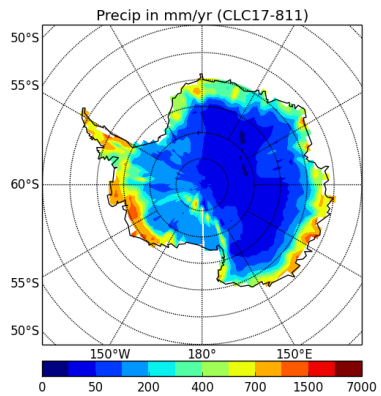
precipSH-CLC17-811
