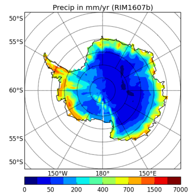
precipSH-RIM1607b
