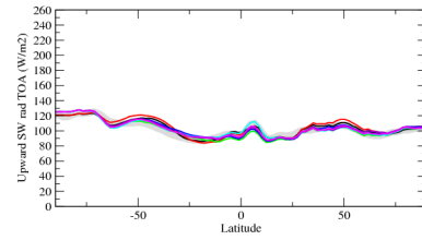
rttsson
