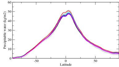
prwazon
