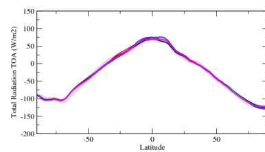
rttsson
