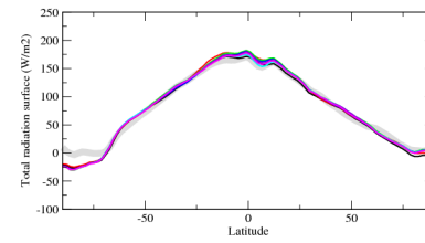
rttsson
