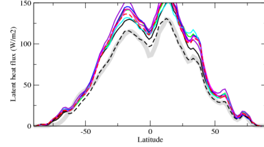
hflszone
