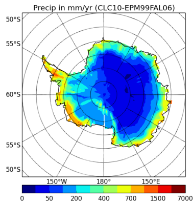
precipSH-CLC10-EPM99FAL06
