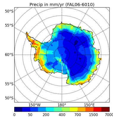
precipSH-FAL06-6010
