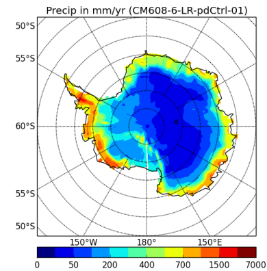
precipSH-CM608-6-LR-pdCtrl-01
