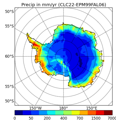
precipSH-CLC22-EPM99FAL06
