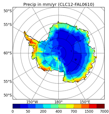
precipSH-CLC12-FAL0610
