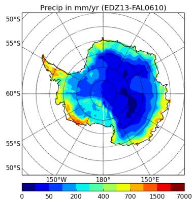
precipSH-EDZ13-FAL0610
