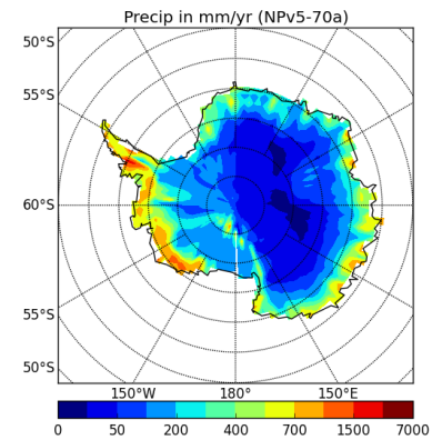
precipSH-NPv5-70a
