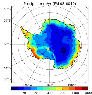
precipSH-FAL08-6010
