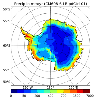
precipSH-CM608-6-LR-pdCtrl-01
