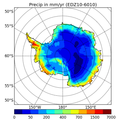
precipSH-EDZ10-6010
