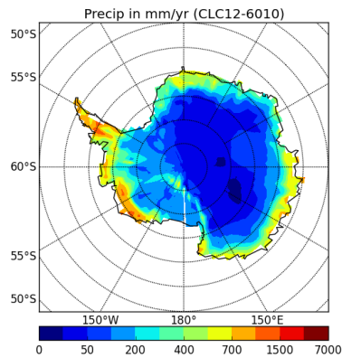
precipSH-CLC12-6010
