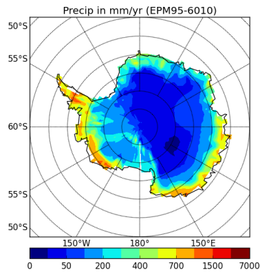
precipSH-EPM95-6010
