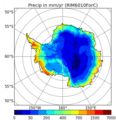
precipSH-RIM6010ForC
