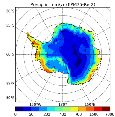
precipSH-EPM75-Ref2
