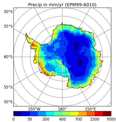
precipSH-EPM99-6010
