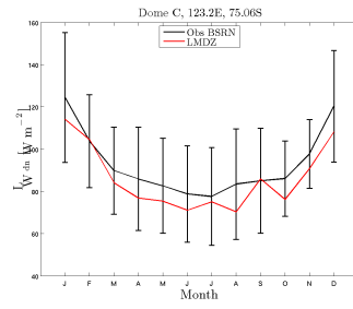
LWdn_DC_RIM601Ofast_1987_1987
