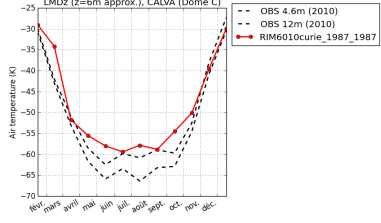
tempDC-RIM601ocurie_1987_1987
