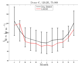
LWdn_DC_RIM601ocurie_1987_1987
