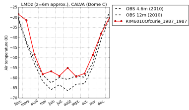
tempDC-RIM601Ofcurie_1987_1987
