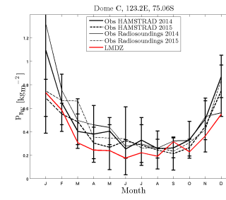
prw_DC_RIM601Ofast_1987_1987
