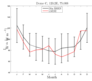
LWdn_DC_RIM6010ForC_1987_1987
