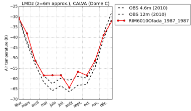
tempDC-RIM601Ofada_1987_1987
