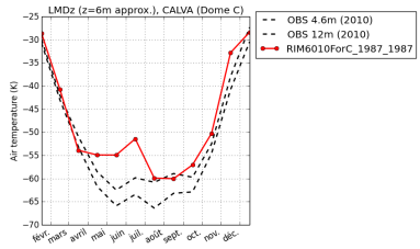
tempDC-RIM6010ForC_1987_1987
