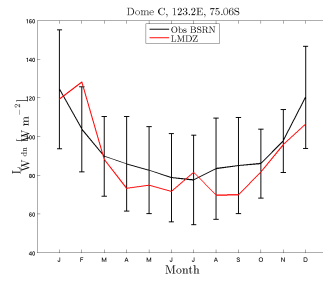
LWdn_DC_RIM601Ofcurie_1987_1987
