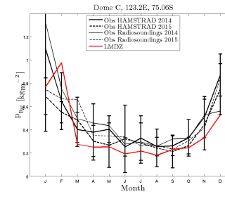
prw_DC_RIM601ocurie_1987_1987
