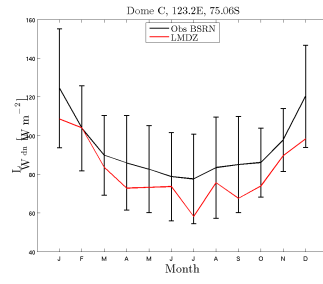
LWdn_DC_RIM601Ofada_1987_1987
