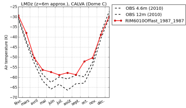
tempDC-RIM601Ofast_1987_1987
