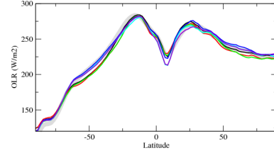
rlutzon
