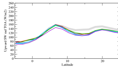
rstzcn
