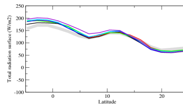
rtzcn
