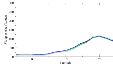
rsuszcn
