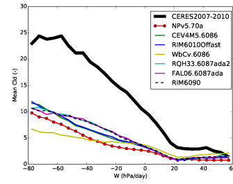
clmcalipso_Tun6086
