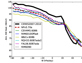
rsah_Tun6086
