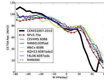
rttcs_Tun6086
