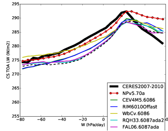
rlutcs_Tun6086
