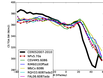
rsttcs_Tun6086
