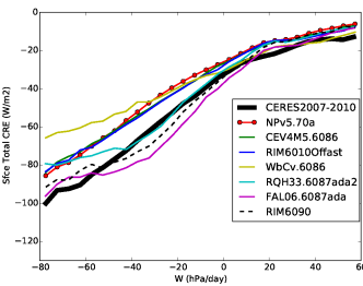
crets_Tun6086
