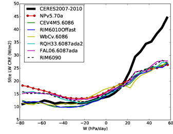
crels_Tun6086
