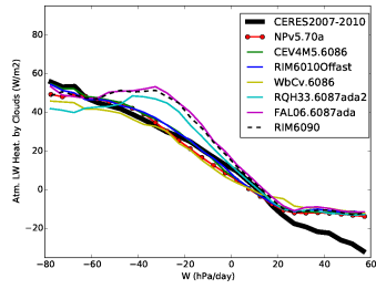
rlahcre_Tun6086
