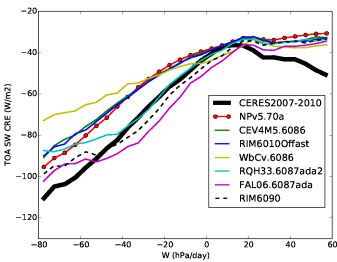
crest_Tun6086
