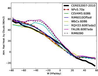
rahcre_Tun6086
