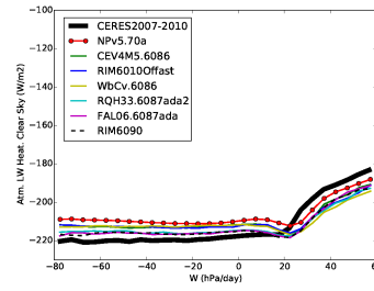
rlahcs_Tun6086
