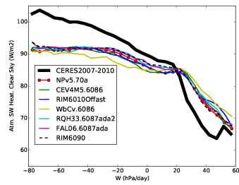
rsahcs_Tun6086
