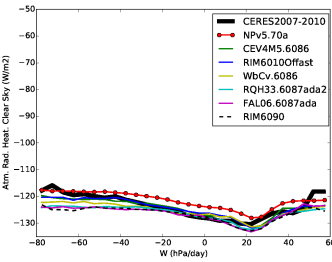
rahcs_Tun6086
