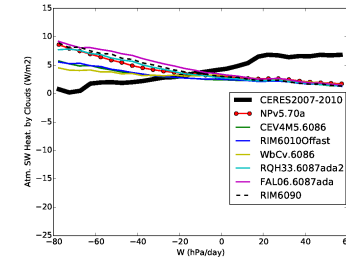
rsahcre_Tun6086
