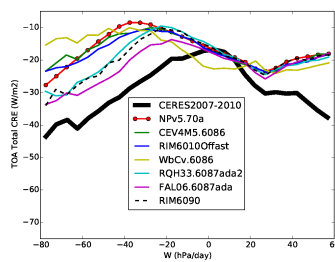
crett_Tun6086
