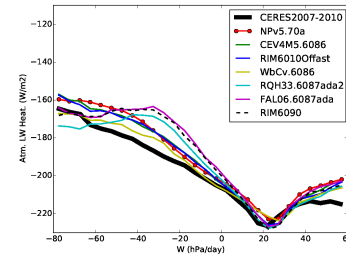
rlah_Tun6086
