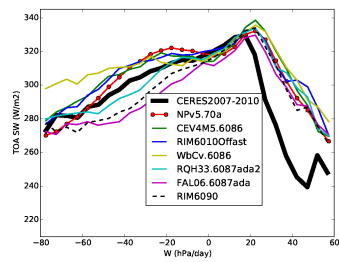
rstt_Tun6086
