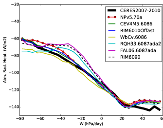
rah_Tun6086
