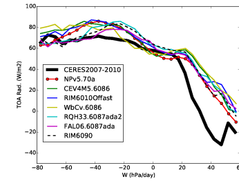
rtt_Tun6086
