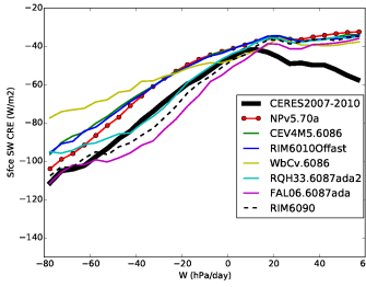
cross_Tun6086
