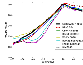
rlut_Tun6086
