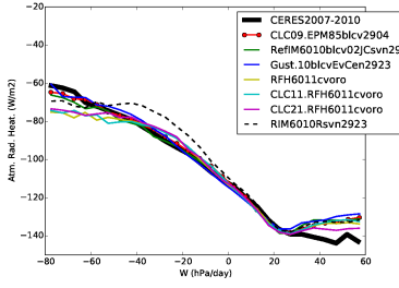
rah_Tun6011cvoro
