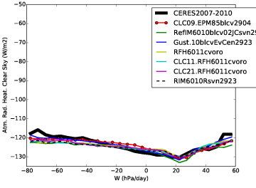
rahcs_Tun6011cvoro
