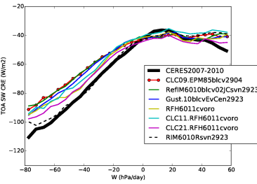
crest_Tun6011cvoro
