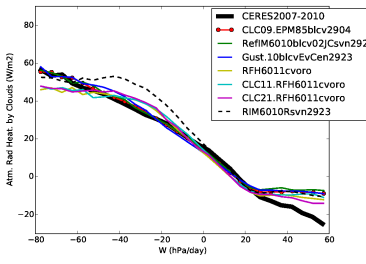
rahcre_Tun6011cvoro
