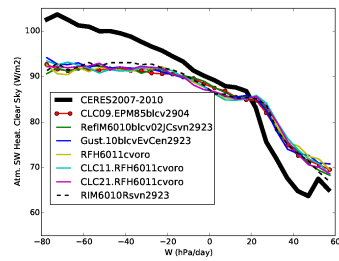
rsahcs_Tun6011cvoro
