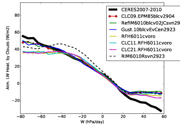
rlahcre_Tun6011cvoro
