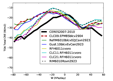
crett_Tun6011cvoro
