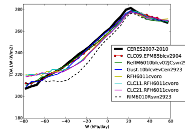
rlut_Tun6011cvoro
