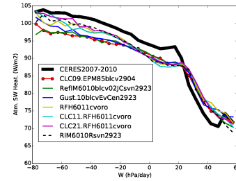
rsah_Tun6011cvoro
