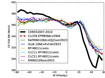
rstcs_Tun6011cvoro
