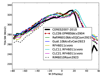
rstt_Tun6011cvoro
