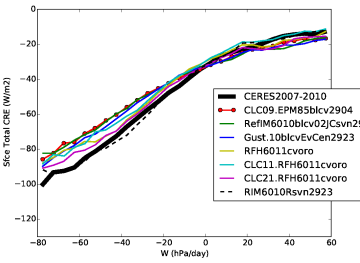
crets_Tun6011cvoro
