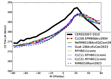
rlutcs_Tun6011cvoro
