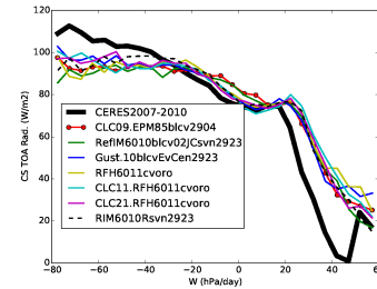
rttcs_Tun6011cvoro
