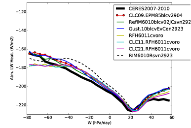
rlah_Tun6011cvoro
