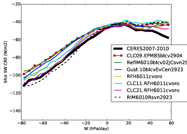
cross_Tun6011cvoro
