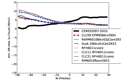
rsahcre_Tun6011cvoro
