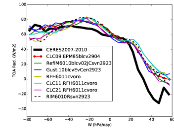
rtt_Tun6011cvoro
