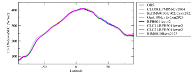
rldscrezon
