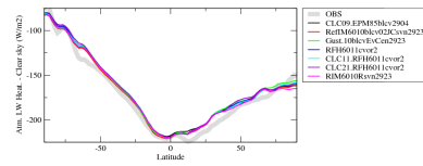
rlahczson
