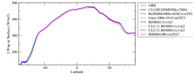
rluscrezon
