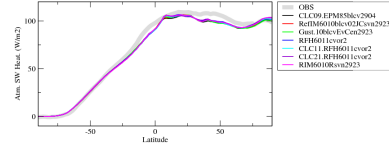
rsahczson
