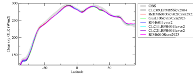
rlutcrezon
