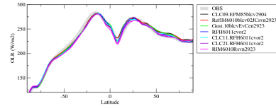
rlutczson
