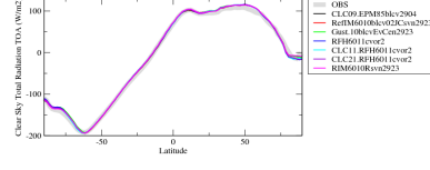
rttcrezon
