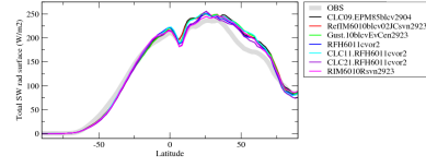
rsdscrezon
