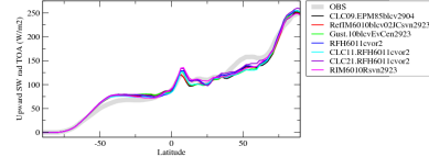
rsutczson
