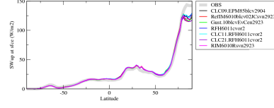
rsuscrezon
