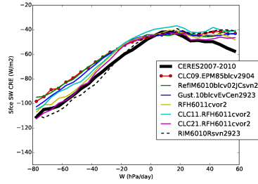
cross_Tun6011cvor2
