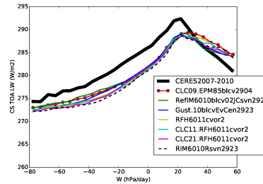
rlutcs_Tun6011cvor2
