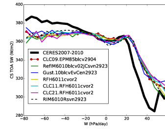
rsttcs_Tun6011cvor2
