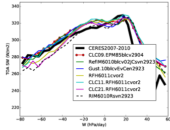
rstt_Tun6011cvor2
