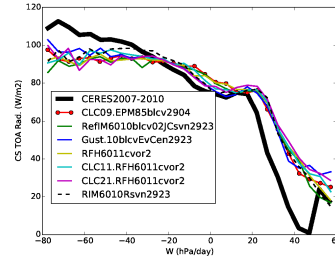
rtctcs_Tun6011cvor2
