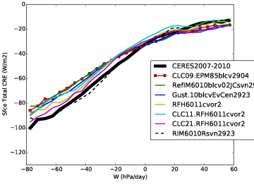
cretst_Tun6011cvor2
