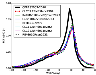
ww_Tun6011cvor2
