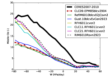
clmcalipso_Tun6011cvor2
