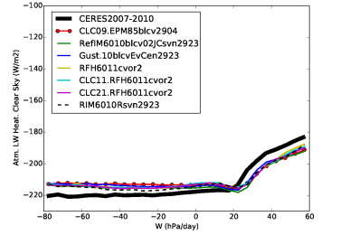
rlahcs_Tun6011cvor2
