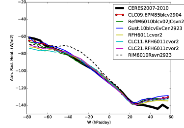
rah_Tun6011cvor2
