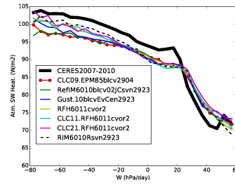
rsah_Tun6011cvor2
