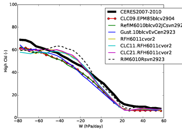
clhcalipso_Tun6011cvor2
