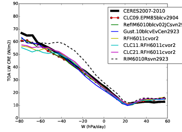
cretl_Tun6011cvor2
