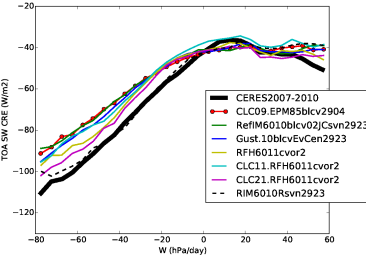
crest_Tun6011cvor2
