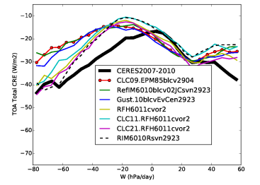
crettt_Tun6011cvor2
