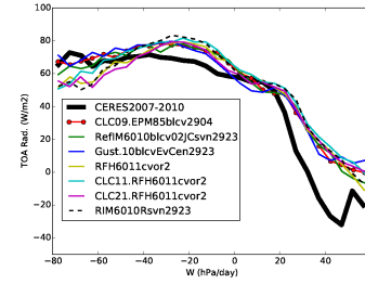
rtt_Tun6011cvor2
