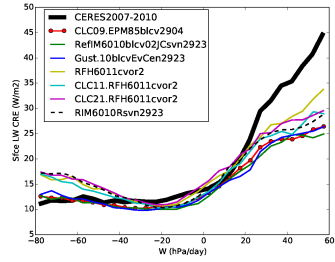
crels_Tun6011cvor2
