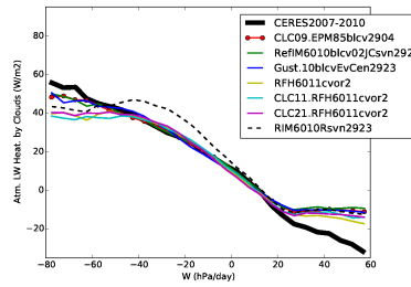
rlahcre_Tun6011cvor2
