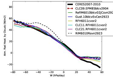
rahcre_Tun6011cvor2
