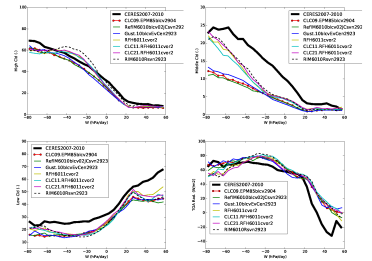
REG_Tun6011cvor2_Tuning-0
