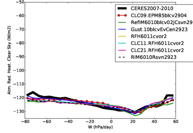
rahcs_Tun6011cvor2
