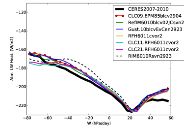
rlah_Tun6011cvor2
