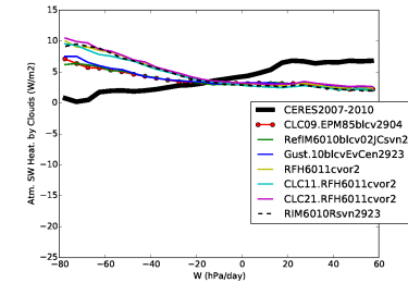
rsahcre_Tun6011cvor2
