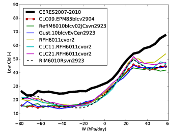
cllcalipso_Tun6011cvor2
