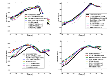
REG_Tun6011cvor2_Tuning-1
