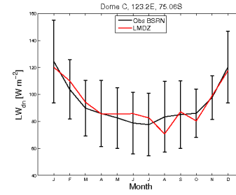
LWdnSFC_DC_RadCv2Fiz.RIV104_1987_1987
