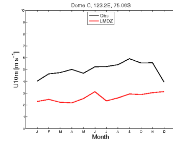
wind10m_DC_RIV60103b2878
