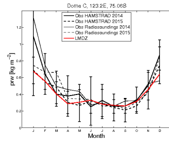
prw_DC_CM608.6-LR-pdCtrl-01_2040_2049
