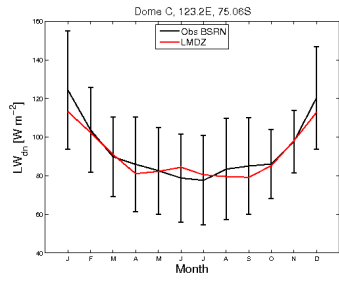
LWdnSFC_DC_CM608.6-LR-pdCtrl-01_2040_2049
