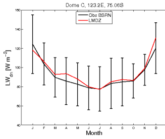
LWdnSFC_DC_RIV60103b2878_1987_1987
