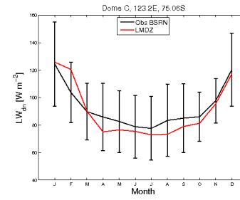
LWdnSFC_DC_CLC12.6010_1987_1987
