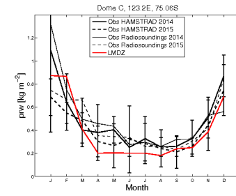
prw_DC_CLC12.6010_1987_1987
