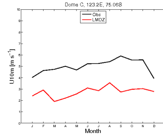
wind10m_DC_RIV60104_1987_1987
