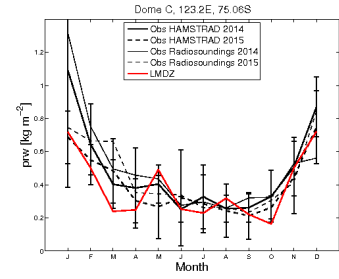
prw_DC_RIV60104_1987_1987
