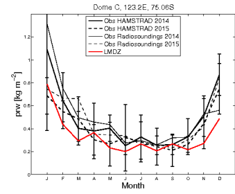
prw_DC_EPM98.FAL0610_1987_1987
