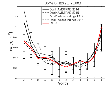
prw_DC_RIV60103b2878_1987_1987
