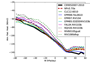
rah_Tun60103falrqh
