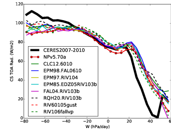
rttcs_Tun60103falrqh
