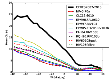
clmcalipso_Tun60103falrqh
