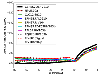
rlahcs_Tun60103falrqh
