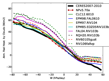
rahcre_Tun60103falrqh
