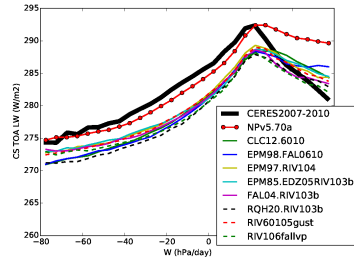
rlutcs_Tun60103falrqh
