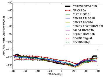
rahcs_Tun60103falrqh
