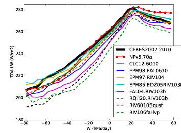
rlut_Tun60103falrqh
