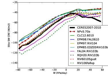
cross_Tun60103falrqh
