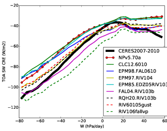
crest_Tun60103falrqh
