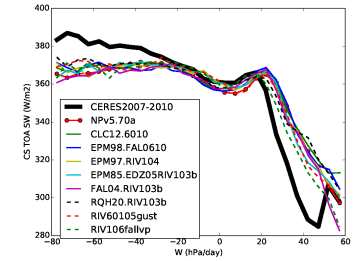
rsttcs_Tun60103falrqh
