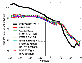
rsahcs_Tun60103falrqh
