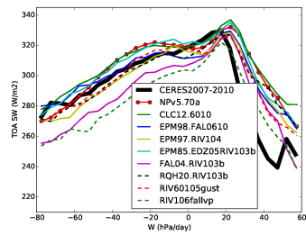
rstt_Tun60103falrqh
