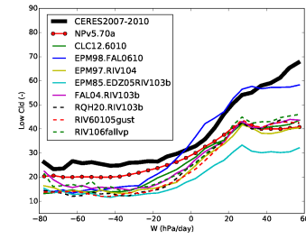
cllcalipso_Tun60103falrqh
