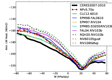
rlah_Tun60103falrqh
