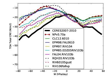
crettt_Tun60103falrqh
