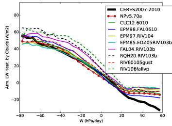
rlahcre_Tun60103falrqh
