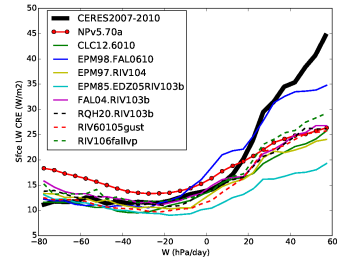
crels_Tun60103falrqh
