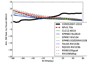
rsahcre_Tun60103falrqh
