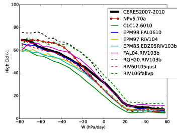
clhcalipso_Tun60103falrqh
