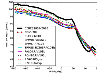
rsah_Tun60103falrqh
