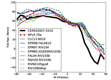
rtt_Tun60103falrqh
