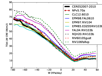
cretl_Tun60103falrqh
