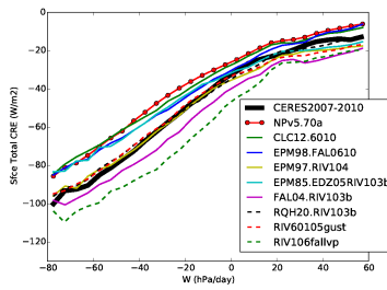
cretst_Tun60103falrqh
