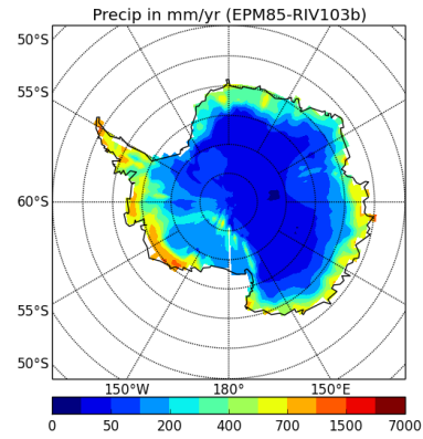
precipSH-EPM85-RIV103b
