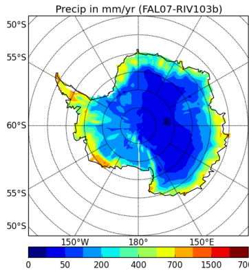
precipSH-FAL07-RIV103b
