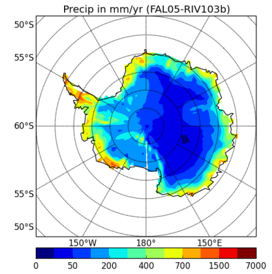
precipSH-FAL05-RIV103b
