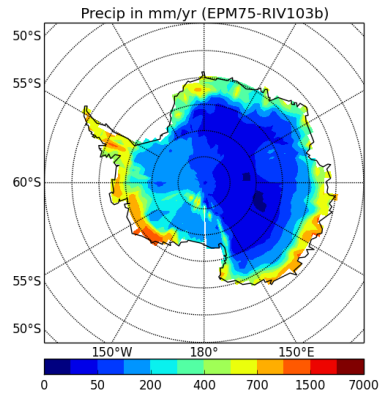
precipSH-EPM75-RIV103b
