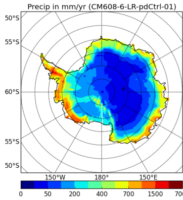
precipSH-CM608-6-LR-pdCtrl-01
