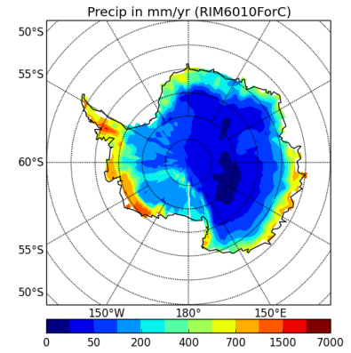
precipSH-RIM6010ForC
