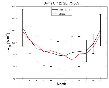
LWdnSFC_DC_EDZ09.RIV103b_1987_1987
