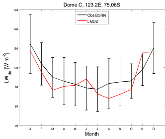
LWdnSFC_DC_RIM6010ForC_1987_1987
