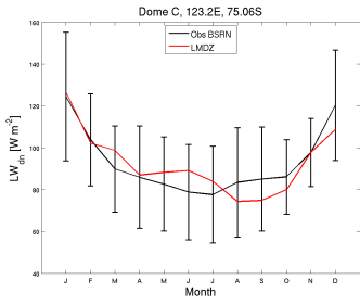
LWdnSFC_DC_RIV60103b_1987_1987
