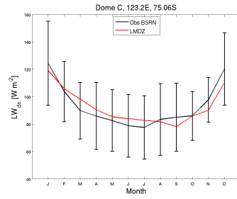
LWdnSFC_DC_CLC15.RIV103b_1987_1987
