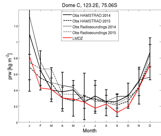
prw_DC_CLC09.RIV103b_1987_1987
