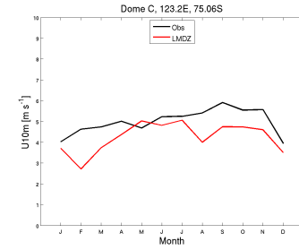
wind10m_DC_RIM6010ForC_1987_1987
