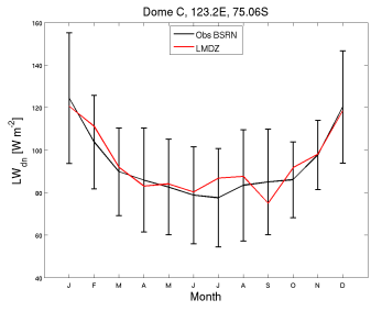
LWdnSFC_DC_EDZ05.RIV103b_1987_1987
