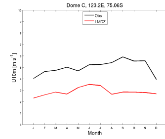
wind10m_DC_RIV60103b_1987_1987
