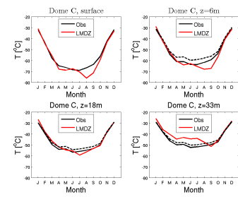
temp_DC_RIV60103b_1987_1987
