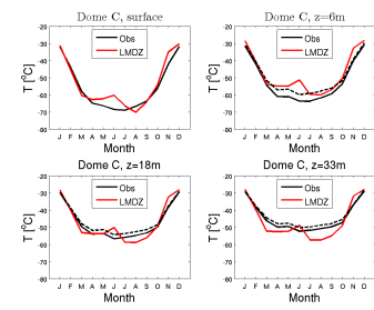
temp_DC_RIM6010ForC_1987_1987
