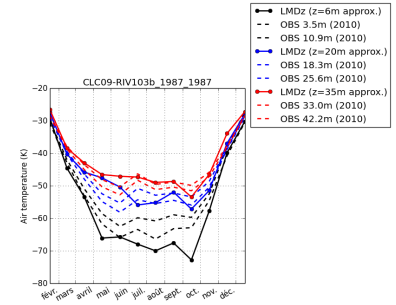
tempDC-CLC09-RIV103b_1987_1987
