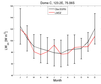
LWdnSFC_DC_CDO1.RIV103b_1987_1987
