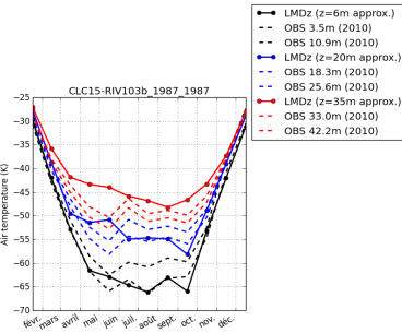
tempDC-CLC15-RIV103b_1987_1987
