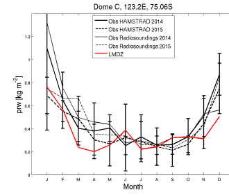
prw_DC_CDO1.RIV103b_1987_1987
