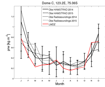
prw_DC_RIM6010ForC_1987_1987
