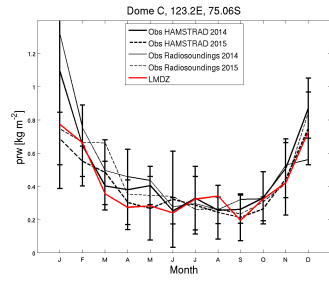
prw_DC_EDZ05.RIV103b_1987_1987
