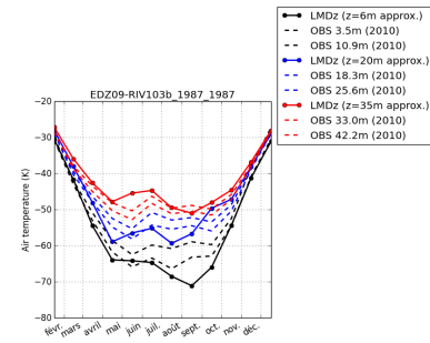
tempDC-EDZ09-RIV103b_1987_1987
