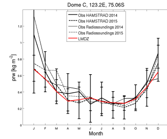
prw_DC_CM608.6-LR-pdCtrl-01_2040_2049
