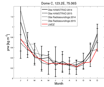
prw_DC_CLC15.RIV103b_1987_1987
