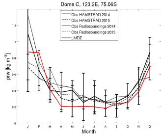
prw_DC_CLC12.6010_1987_1987
