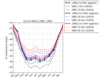
tempDC-CLC12-6010_1987_1987
