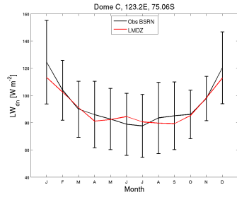
LWdnSFC_DC_CM608.6-LR-pdCtrl-01_2040_2049
