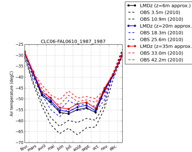
tempDC-CLC06-FAL0610_1987_1987
