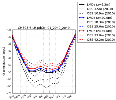
tempDC-CM608-6-LR-pdCtrl-01_2040_2049
