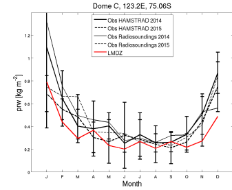
prw_DC_EPM98.FAL0610_1987_1987
