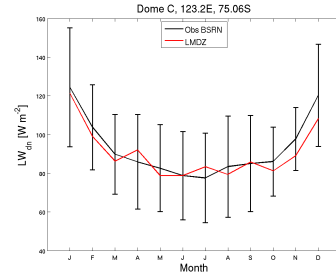
LWdnSFC_DC_EPM98.FAL0610_1987_1987
