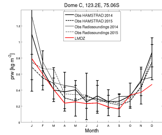
prw_DC_CLC09.FAL0610_1987_1987
