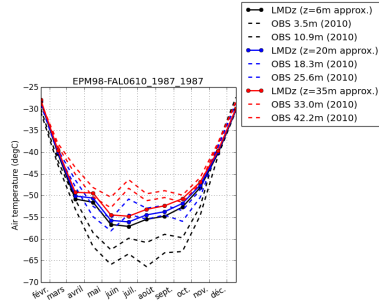
tempDC-EPM98-FAL0610_1987_1987
