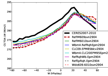
rlutcs_Tun10wbrqh
