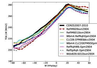
rlut_Tun10wbrqh
