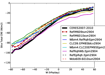
crets_Tun10wbrqh
