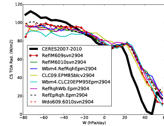
rttcs_Tun10wbrqh
