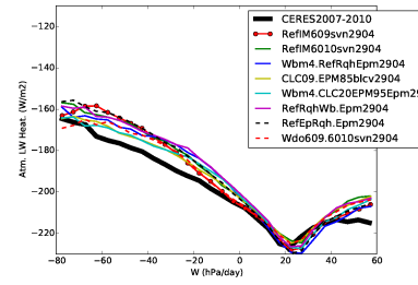
rlah_Tun10wbrqh
