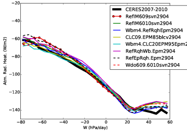
rah_Tun10wbrqh
