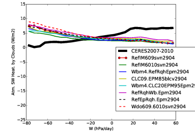
rsahcre_Tun10wbrqh
