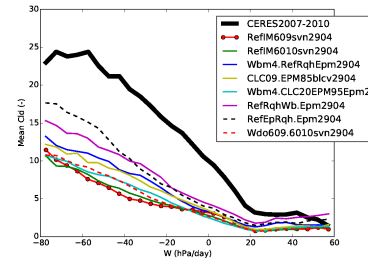
clmcalipso_Tun10wbrqh
