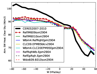
rsahcs_Tun10wbrqh
