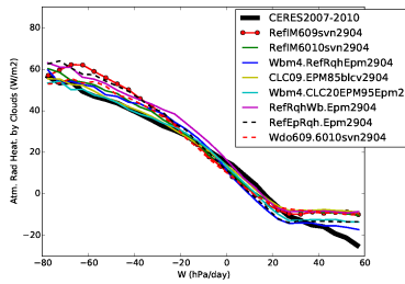
rahcre_Tun10wbrqh
