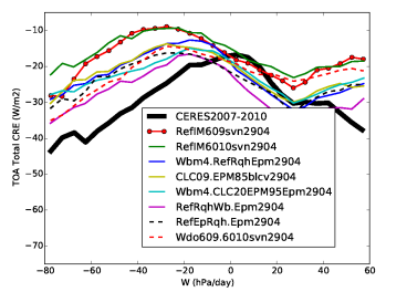
crett_Tun10wbrqh
