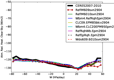
rahcs_Tun10wbrqh
