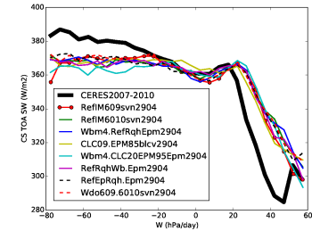
rsttcs_Tun10wbrqh
