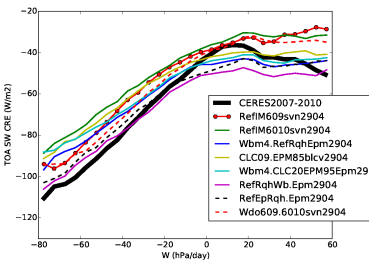
crest_Tun10wbrqh
