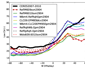
cllcalipso_Tun10wbrqh
