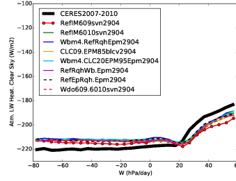
rlahcs_Tun10wbrqh
