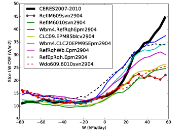
crels_Tun10wbrqh
