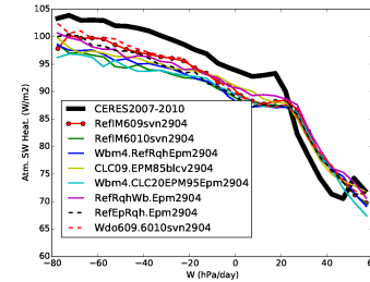
rsah_Tun10wbrqh
