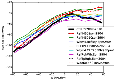
cross_Tun10wbrqh
