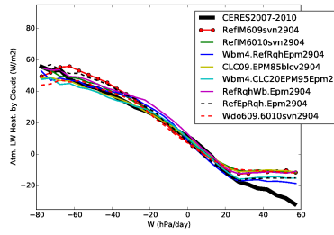
rlahcre_Tun10wbrqh
