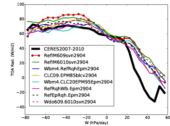
rtt_Tun10wbrqh
