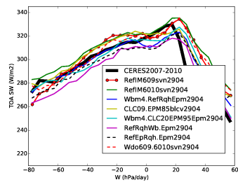
rstt_Tun10wbrqh
