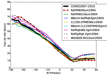
cretl_Tun10wbrqh
