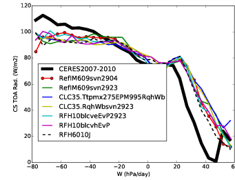
rttcs_Tun10svn2923CR
