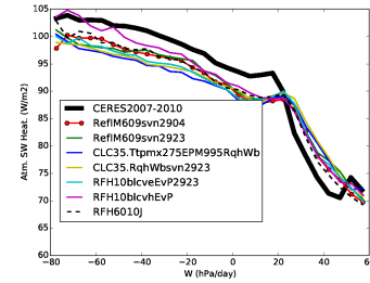
rsah_Tun10svn2923CR
