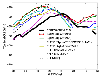
crettt_Tun10svn2923CR
