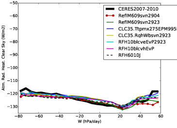
rahcs_Tun10svn2923CR
