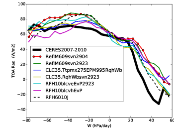
rtt_Tun10svn2923CR
