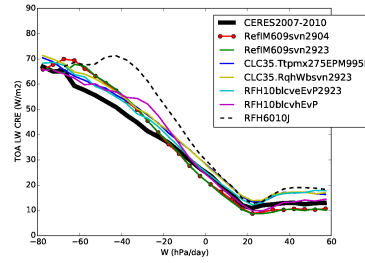
cretl_Tun10svn2923CR
