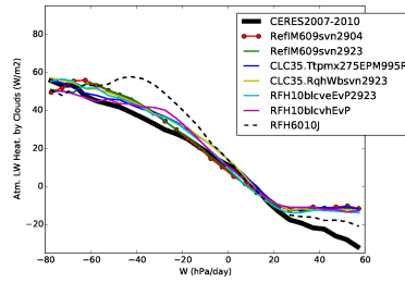
rlahcre_Tun10svn2923CR
