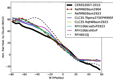
rahcre_Tun10svn2923CR
