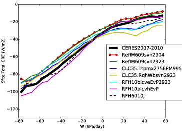
cretst_Tun10svn2923CR
