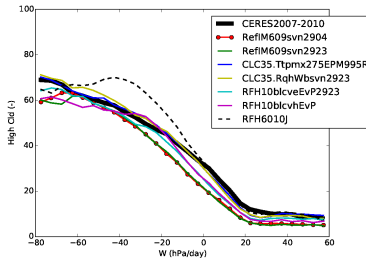
clhcalipso_Tun10svn2923CR
