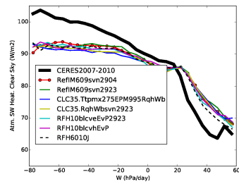
rsahcs_Tun10svn2923CR
