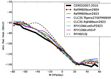
rah_Tun10svn2923CR
