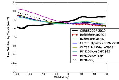
rsahcre_Tun10svn2923CR
