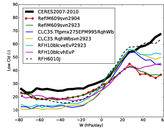
cllcalipso_Tun10svn2923CR
