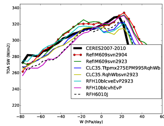
rstt_Tun10svn2923CR
