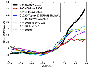
crels_Tun10svn2923CR
