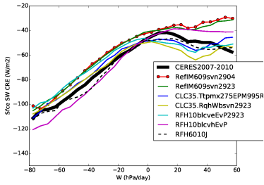
cross_Tun10svn2923CR
