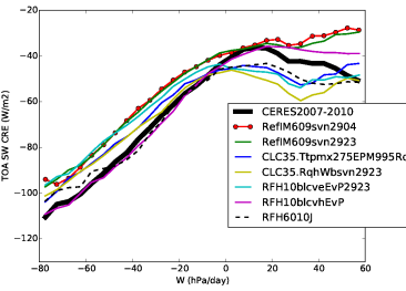
crest_Tun10svn2923CR
