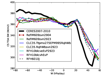
rsttcs_Tun10svn2923CR
