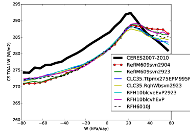
rlutcs_Tun10svn2923CR
