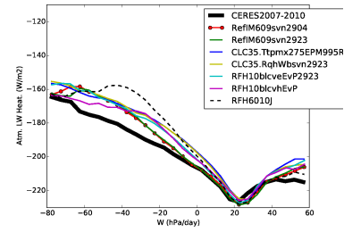
rlah_Tun10svn2923CR
