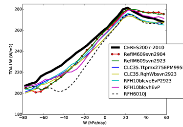
rlut_Tun10svn2923CR
