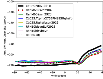
rlahcs_Tun10svn2923CR
