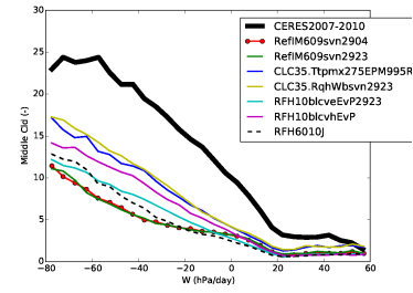
clmcalipso_Tun10svn2923CR
