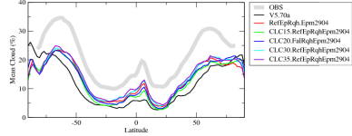
almcalipsozon
