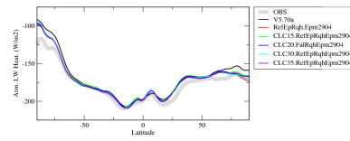
rlahzon
