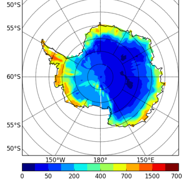
precipSH-CLC20-FalRqhEpm2904
