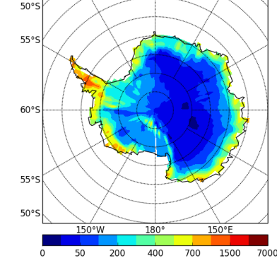
precipSH-RefEpRqh-Epm2904
