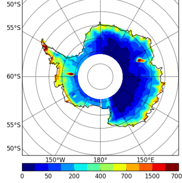
precipSH-OBS
