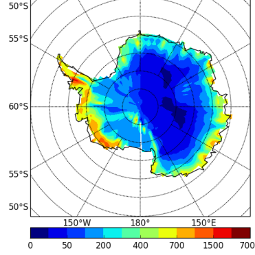
precipSH-NPv5-70a
