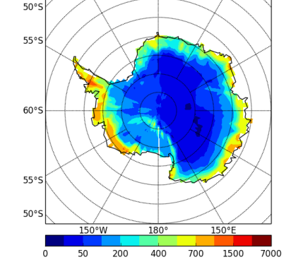
precipSH-CLC35-RefEpRqhEpm2904
