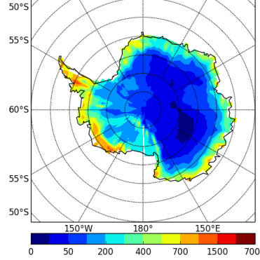
precipSH-CLC15-RefEpRqhEpm2904
