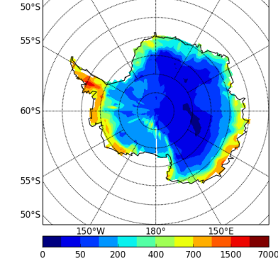
precipSH-CLC30-RefEpRqhEpm2904
