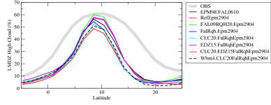
clhson
