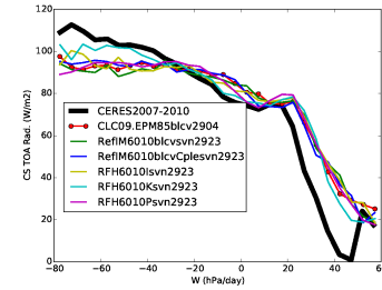
rttcs_Tun10blcvIKP
