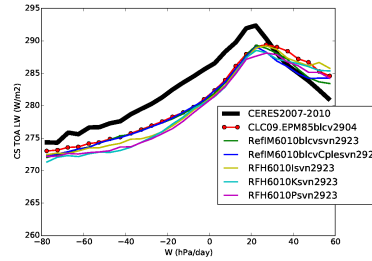
rlutcs_Tun10blcvIKP
