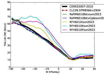
crelt_Tun10blcvIKP
