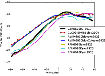
crest_Tun10blcvIKP
