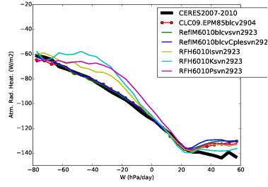
rah_Tun10blcvIKP
