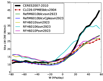
crels_Tun10blcvIKP
