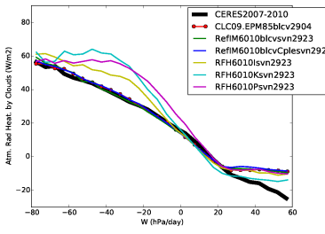
rahcre_Tun10blcvIKP
