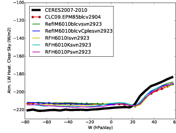
rlahcs_Tun10blcvIKP
