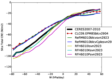
crets_Tun10blcvIKP
