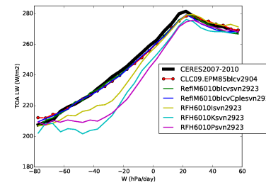
rlut_Tun10blcvIKP
