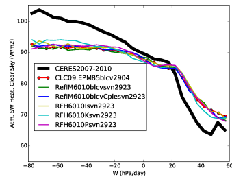
rsahcs_Tun10blcvIKP
