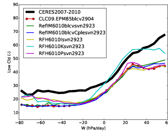
cllcalipso_Tun10blcvIKP
