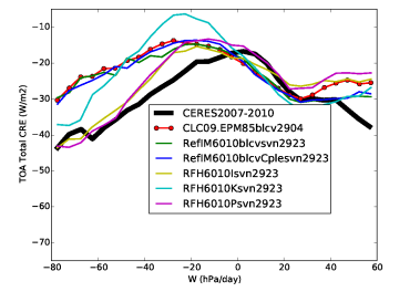
cretT_Tun10blcvIKP
