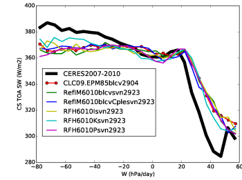
rsttcs_Tun10blcvIKP
