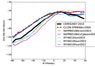
cross_Tun10blcvIKP
