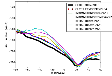
rlah_Tun10blcvIKP
