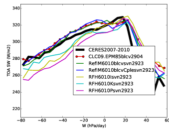
rstt_Tun10blcvIKP
