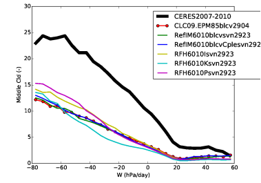
clmcalipso_Tun10blcvIKP
