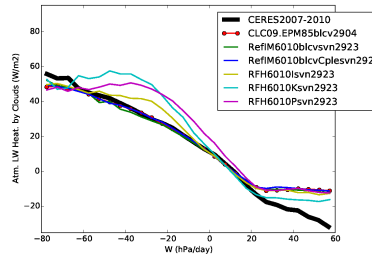
rlahcre_Tun10blcvIKP
