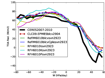
rtt_Tun10blcvIKP
