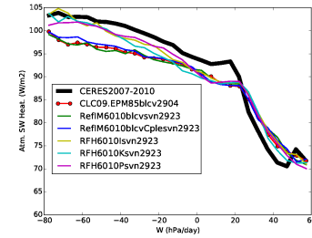
rsah_Tun10blcvIKP
