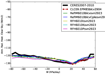
rahcs_Tun10blcvIKP
