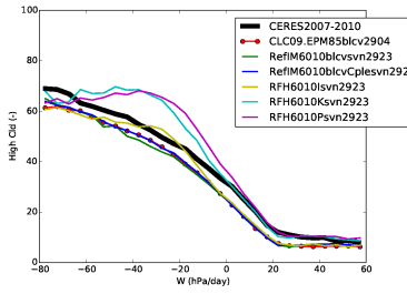
cllcalipso_Tun10blcvIKP
