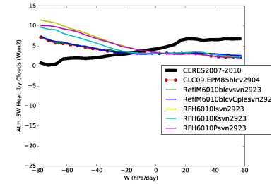
rsahcre_Tun10blcvIKP
