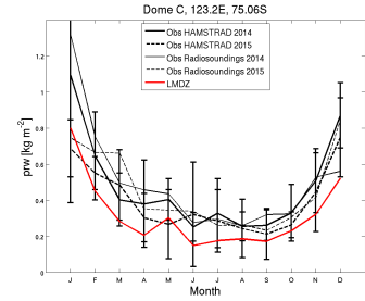
prw_DC_RefIM6010blcvsvn2923_1987_1987
