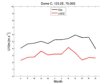
wind10m_DC_RFH6010Isvn2923_1987_1987
