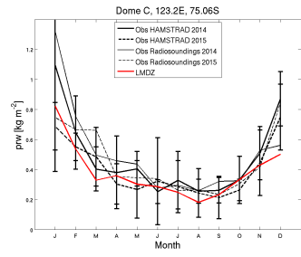
prw_DC_RFH6010Ksvn2923_1987_1987
