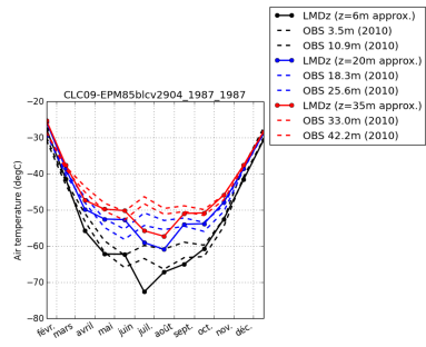
tempDC-CLC09-EPM85blcv2904_1987_1987
