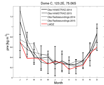
prw_DC_RefIM6010blcvCplesvn2923_1987_1987
