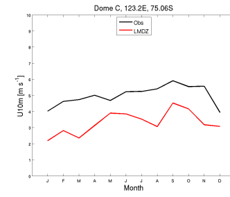
wind10m_DC_RFH6010Ksvn2923_1987_1987
