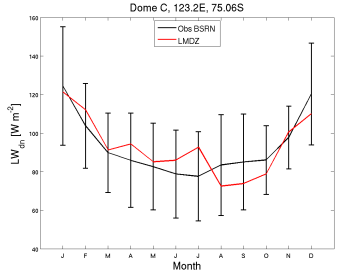
LWdnSFC_DC_RFH6010Psvn2923_1987_1987
