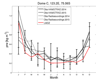
prw_DC_RFH6010Isvn2923_1987_1987
