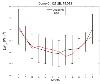
LWdnSFC_DC_RFH6010Ksvn2923_1987_1987
