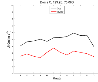
wind10m_DC_RFH6010Psvn2923_1987_1987
