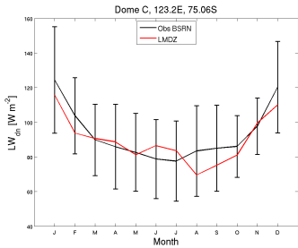
LWdnSFC_DC_RefIM6010blcvCplesvn2923_1987_1987
