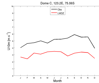
wind10m_DC_RefIM6010blcvCplesvn2923_1987_1987
