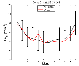
LWdnSFC_DC_Ttpmx275.EPM99RqhWbEpm2904_1987_1987
