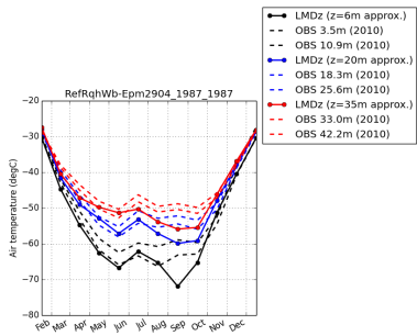
tempDC-RefRqhWb-Epm2904_1987_1987
