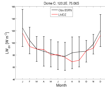
LWdnSFC_DC_RefRqhWb.Epm2904_1987_1987
