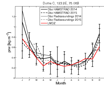
prw_DC_Ttpmx265.EPM995RqhWbEpm2904_1987_1987
