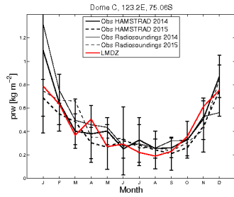
prw_DC_Ttpmx265.EPM99RqhWbEpm2904_1987_1987
