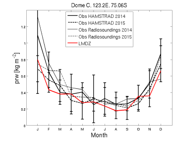
prw_DC_RefRqhWb.Epm2904_1987_1987
