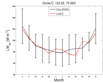
LWdnSFC_DC_EPM99.RqhWbEpm2904_1987_1987
