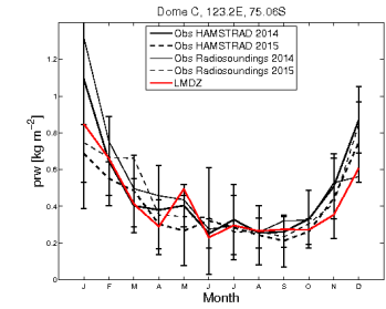
prw_DC_Ttpmx275.EPM99RqhWbEpm2904_1987_1987
