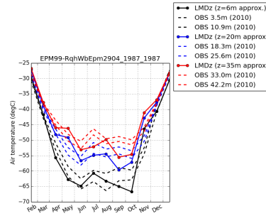
tempDC-EPM99-RqhWbEpm2904_1987_1987
