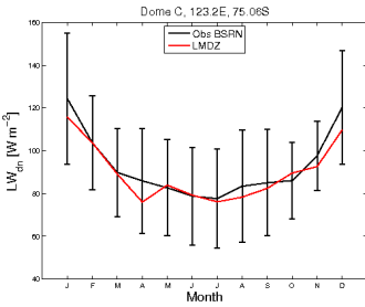
LWdnSFC_DC_Ttpmx265.EPM995RqhWbEpm2904_1987_1987
