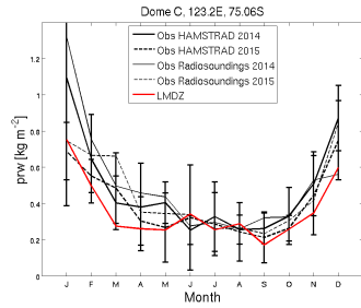
prw_DC_NOtopmx.Wbm4RqhEpm2904_1987_1987
