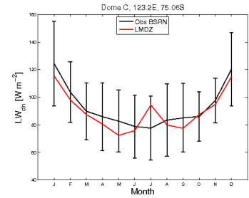
LWdnSFC_DC_Ttpmx275.EPM995RqhWbEpm2904_1987_1987
