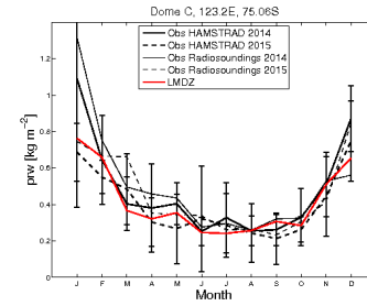
prw_DC_CLC30.Wbm4RqhEpm2904_1987_1987
