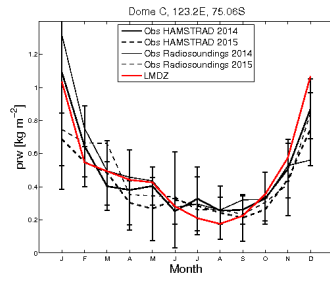
prw_DC_RefIM609svn2904_1987_1987
