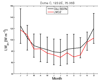
LWdnSFC_DC_CLC20.Wbm4RqhEpm2904_1987_1987
