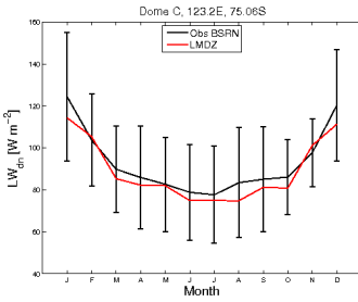
LWdnSFC_DC_CLC30.Wbm4RqhEpm2904_1987_1987
