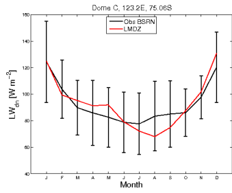
LWdnSFC_DC_RefIM609svn2904_1987_1987
