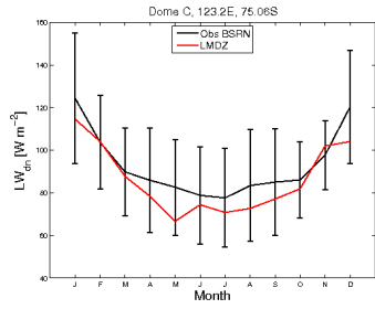
LWdnSFC_DC_CLC15.Wbm4RqhEpm2904_1987_1987
