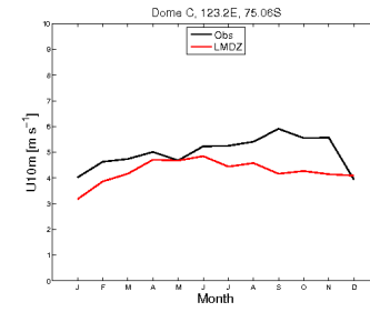
wind10m_DC_RefIM609svn2904_1987_1987
