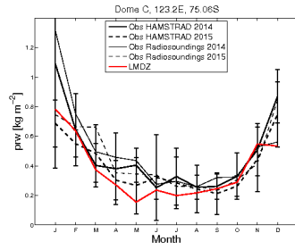
prw_DC_CLC15.Wbm4RqhEpm2904_1987_1987
