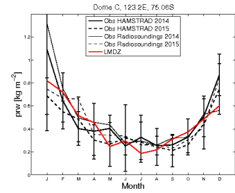
prw_DC_Wbm4.RefRqhEpm2904_1987_1987
