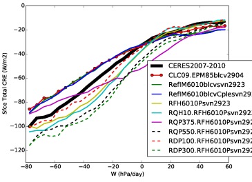
crets_Tun10FHPrqhp
