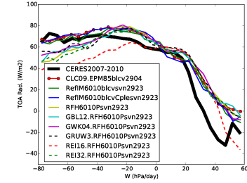
rtt_Tun10FHPrqhp
