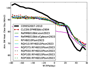
rsahcs_Tun10FHPrqhp
