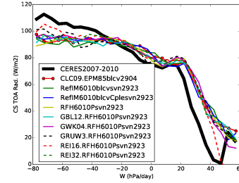
rttcs_Tun10FHPrqhp
