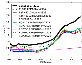
cllcalipso_Tun10FHPrqhp
