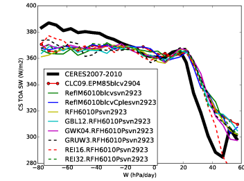
rstcs_Tun10FHPrqhp
