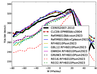
rstt_Tun10FHPrqhp
