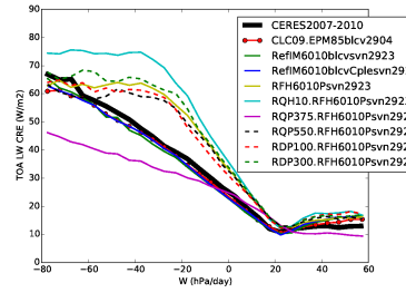
cretl_Tun10FHPrqhp
