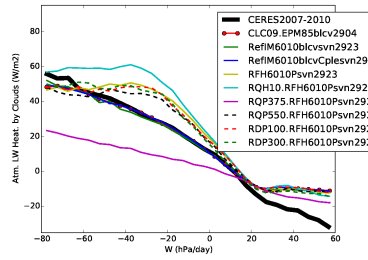
rlahcre_Tun10FHPrqhp
