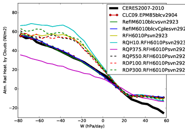
rahcre_Tun10FHPrqhp
