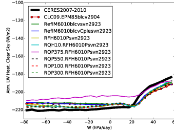
rlahcs_Tun10FHPrqhp
