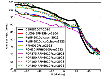
rsah_Tun10FHPrqhp
