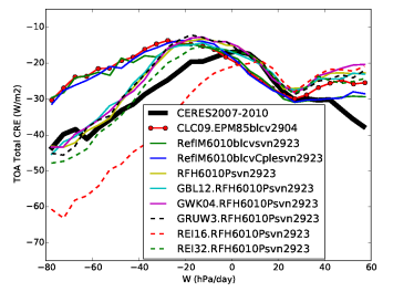
crett_Tun10FHPrqhp
