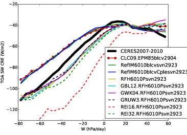
crest_Tun10FHPrqhp
