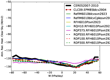
rahcs_Tun10FHPrqhp
