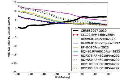
rsahcre_Tun10FHPrqhp
