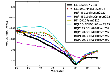
rlah_Tun10FHPrqhp
