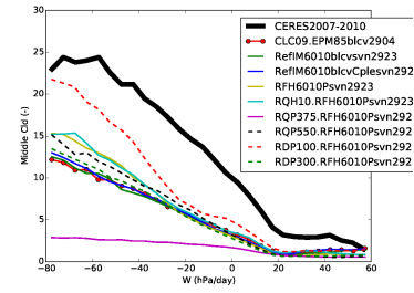
clmcalipso_Tun10FHPrqhp
