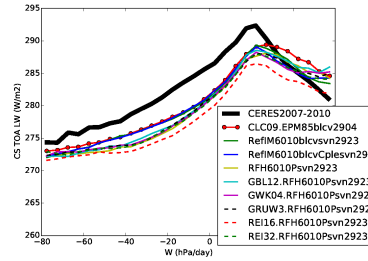
rlutcs_Tun10FHPrqhp
