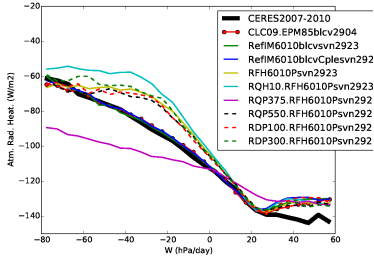
rah_Tun10FHPrqhp
