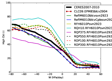
chlcalipso_Tun10FHPrqhp
