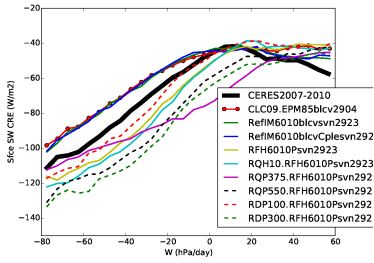
cross_Tun10FHPrqhp
