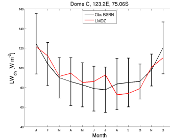
LWdnSFC_DC_RFH6010Psvn2923_1987_1987
