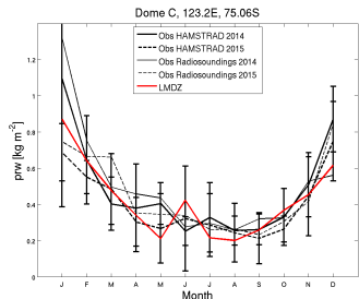
prw_DC_RDP100.RFH6010Psvn2923_1987_1987
