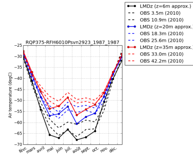
tempDC_RQP375.RFH6010Psvn2923_1987_1987
