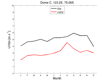
wind10m_DC_RefIM6010blcvsvn2923_1987_1987
