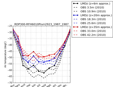
tempDC_RDP300.RFH6010Psvn2923_1987_1987
