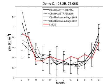
prw_DC_RDP300.RFH6010Psvn2923_1987_1987
