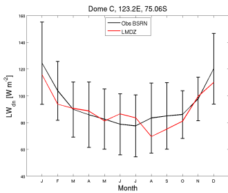
LWdnSFC_DC_RefIM6010blcvCplesvn2923_1987_1987
