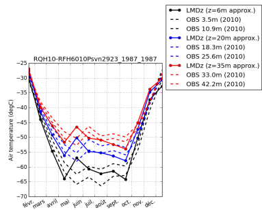
tempDC-RQH10-RFH6010Psvn2923_1987_1987
