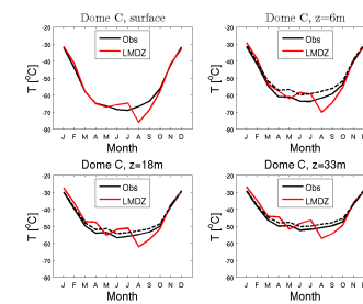
temp_DC_RFH6010Psvn2923_1987_1987
