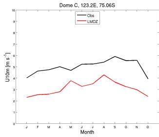
wind10m_DC_RQH10.RFH6010Psvn2923_1987_1987
