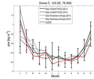
prw_DC_CLC09.EPM85blcv2904_1987_1987
