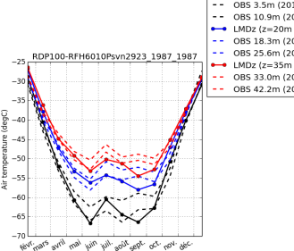
tempDC_RDP100.RFH6010Psvn2923_1987_1987
