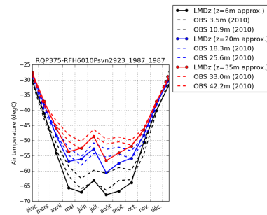
tempDC-RQP375-RFH6010Psvn2923_1987_1987
