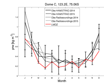
prw_DC_RQP550.RFH6010Psvn2923_1987_1987
