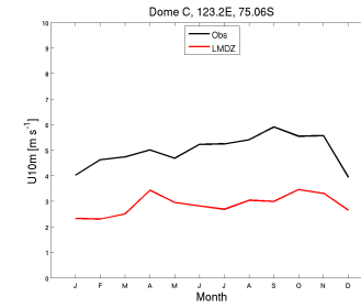
wind10m_DC_RQP550.RFH6010Psvn2923_1987_1987
