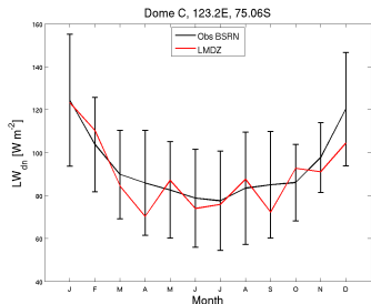
LWdnSFC_DC_RQP550.RFH6010Psvn2923_1987_1987
