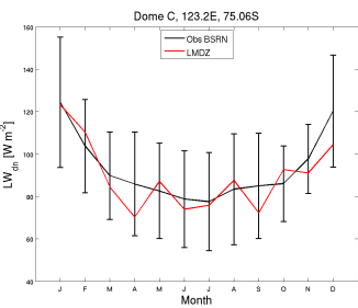
LWdnSFC_DC_RQP550.RFH6010Psvn2923_1987_1987
