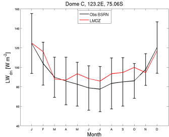
LWdnSFC_DC_RDP300.RFH6010Psvn2923_1987_1987
