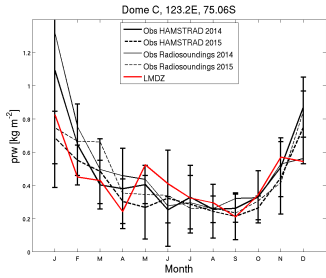
prw_DC_RQH10.RFH6010Psvn2923_1987_1987
