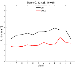
wind10m_DC_RQP375.RFH6010Psvn2923_1987_1987
