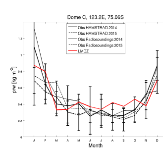
prw_DC_RDP300.RFH6010Psvn2923_1987_1987
