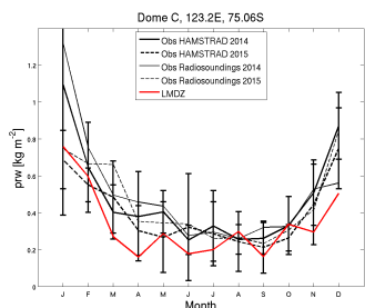
prw_DC_RQP550.RFH6010Psvn2923_1987_1987
