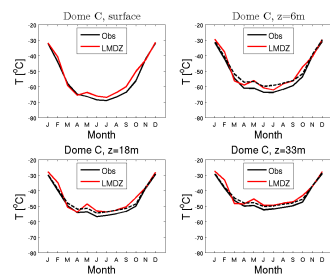
temp_DC_RDP300.RFH6010Psvn2923_1987_1987
