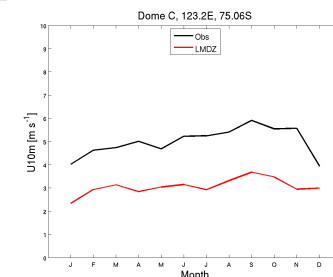
wind10m_DC_RDP100.RFH6010Psvn2923_1987_1987
