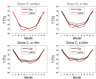
temp_DC_RQP375.RFH6010Psvn2923_1987_1987
