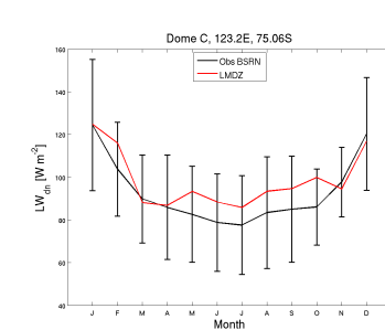
LWdnSFC_DC_RDP300.RFH6010Psvn2923_1987_1987
