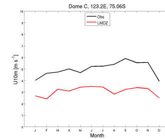
wind10m_DC_RefIM6010blcvCplesvn2923_1987_1987
