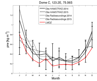
prw_DC_RefIM6010blcvsvn2923_1987_1987
