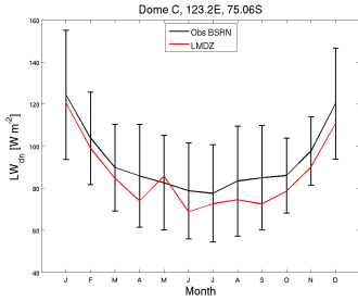
LWdnSFC_DC_RefIM6010blcvsvn2923_1987_1987
