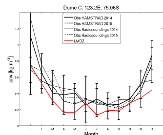
prw_DC_RQP375.RFH6010Psvn2923_1987_1987
