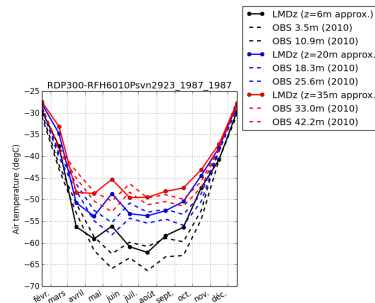
tempDC-RDP300-RFH6010Psvn2923_1987_1987
