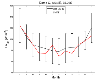
LWdnSFC_DC_RQP375.RFH6010Psvn2923_1987_1987
