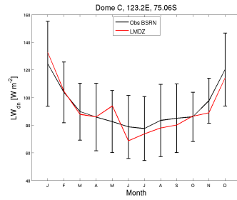
LWdnSFC_DC_CLC09.EPM85blcv2904_1987_1987
