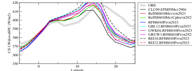
rldscrezon
