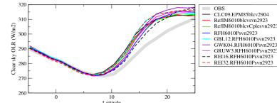
rlutcrezon
