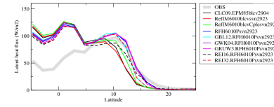
hfnsson
