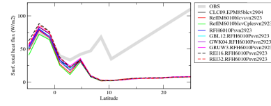
hfnsson
