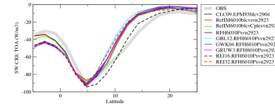
crestzon
