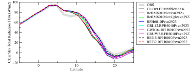
rttcrezon
