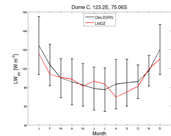
LWdnSFC_DC_RefIM6010blcvCplesvn2923_1987_1987
