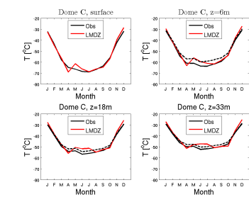
temp_DC_EDZ15.RFH6010Psvn2923_1987_1987
