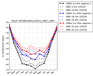
tempDC-FAL07-RFH6010Psvn2923_1987_1987
