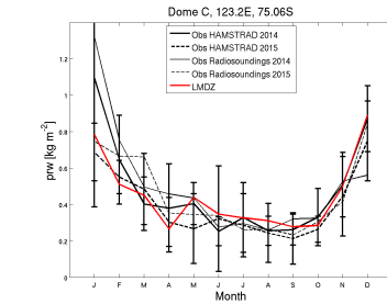
prw_DC_EDZ15.RFH6010Psvn2923_1987_1987
