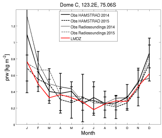
prw_DC_EPM99.RFH6010Psvn2923.1987_1987
