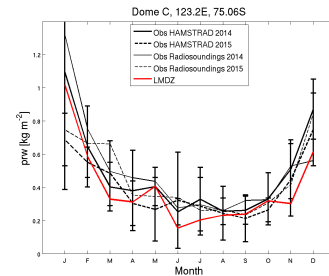
prw_DC_CLC09.EPM85blcv2904_1987_1987
