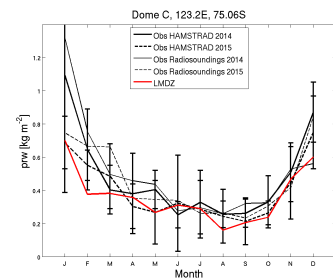
prw_DC_RefIM6010blcvCplesvn2923_1987_1987
