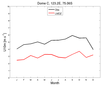
wind10m_DC_FAL07.RFH6010Psvn2923.1987_1987
