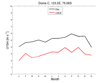
wind10m_DC_Z0QH1.RFH6010Psvn2923.1987_1987
