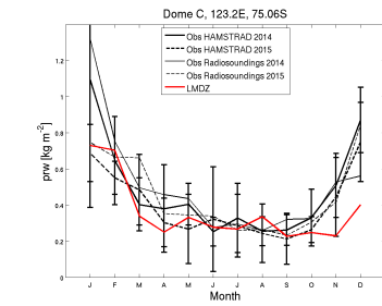
prw_DC_Z0QH1.RFH6010Psvn2923.1987_1987
