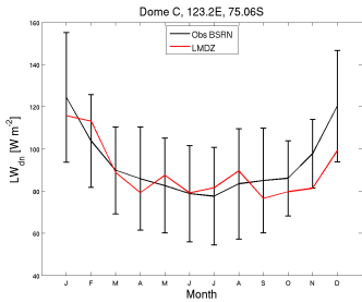
LWdnSFC_DC_Z0QH1.RFH6010Psvn2923_1987_1987
