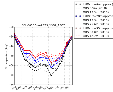
tempDC-RFH6010Psvn2923_1987_1987
