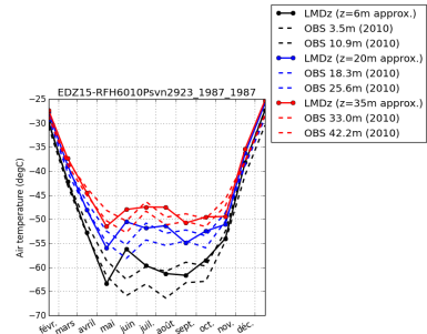
tempDC-EDZ15-RFH6010Psvn2923.1987_1987
