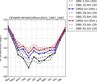
tempDC-CEV6M5-RFH6010Psvn2923.1987_1987
