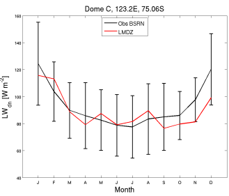
LWdnSFC_DC_Z0QH1.RFH6010Psvn2923.1987_1987
