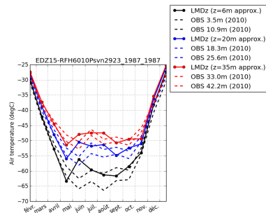
tempDC-EDZ15-RFH6010Psvn2923_1987_1987
