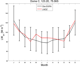
LWdnSFC_DC_EDZ15.RFH6010Psvn2923_1987_1987
