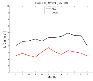
wind10m_DC_RFH6010Psvn2923.1987_1987
