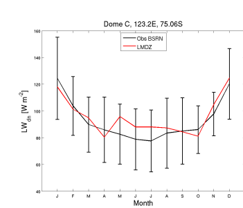
LWdnSFC_DC_EDZ15.RFH6010Psvn2923.1987_1987
