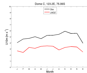
wind10m_DC_RefIM6010blcvCplesvn2923_1987_1987
