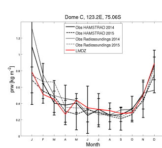
prw_DC_EDZ15.RFH6010Psvn2923.1987_1987
