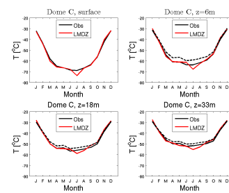
temp_DC_EPM99.RFH6010Psvn2923_1987_1987
