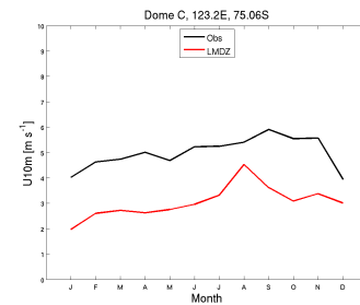
wind10m_DC_RefIM6010blcvsvn2923_1987_1987
