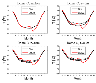
temp_DC_RFH6010Psvn2923_1987_1987
