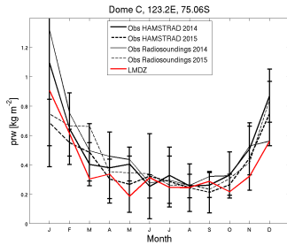
prw_DC_CEV6M5.RFH6010Psvn2923_1987_1987
