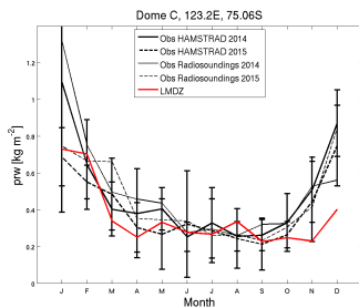
prw_DC_Z0QH1.RFH6010Psvn2923_1987_1987
