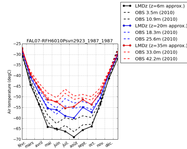
tempDC-FAL07-RFH6010Psvn2923.1987_1987
