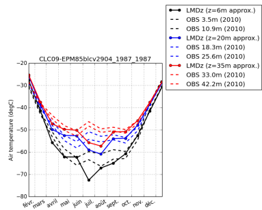
tempDC-CLC09-EPM85blcv2904_1987_1987
