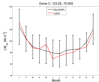
LWdnSFC_DC_CLC09.EPM85blcv2904_1987_1987
