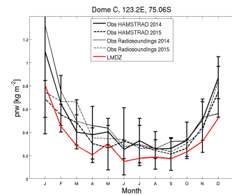
prw_DC_RefIM6010blcvsvn2923_1987_1987
