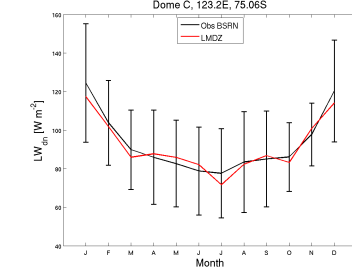
LWdnSFC_DC_EPM99.RFH6010Psvn2923_1987_1987
