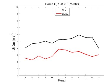
wind10m_DC_CEV6M5.RFH6010Psvn2923_1987_1987
