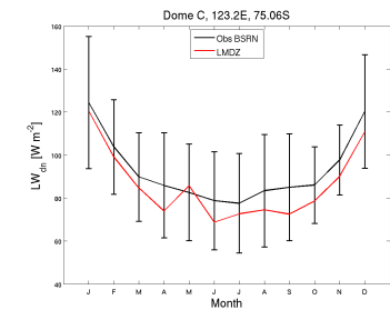
LWdnSFC_DC_RefIM6010blcvsvn2923_1987_1987
