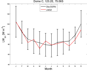
LWdnSFC_DC_CEV6M5.RFH6010Psvn2923_1987_1987
