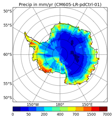
precipSH-CM605-LR-pdCtrl-01
