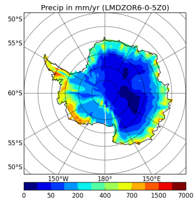
precipSH-LMDZOR6-0-5Z0
