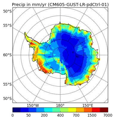
precipSH-CM605-GUST-LR-pdCtrl-01
