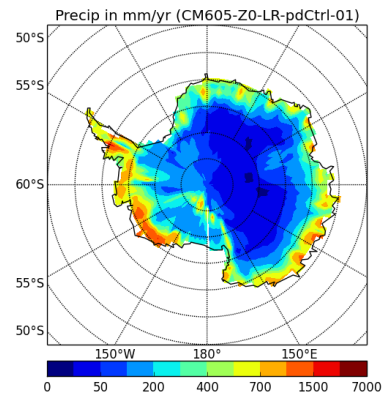
precipSH-CM605-Z0-LR-pdCtrl-01
