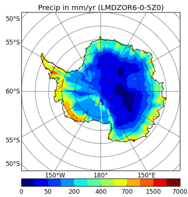
precipSH-LMDZOR6-0-5Z0
