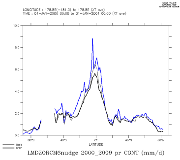
LMDZORCM6nudge_2000_2009_con
