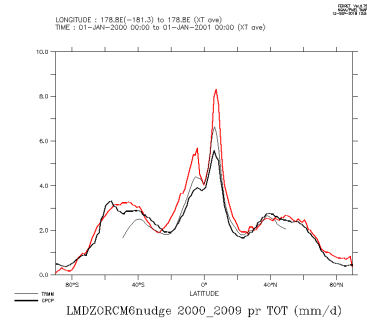
LMDZORCM6nudge_2000_2009_tot
