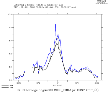
LMDZORnudge.nogustZ0_2000_2009_con
