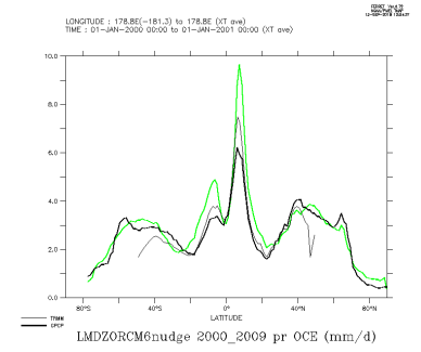
LMDZORCM6nudge_2000_2009_oce
