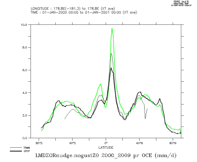
LMDZORnudge.nogustZ0_2000_2009_oce
