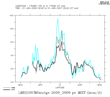
LMDZORCM6nudge_2000_2009_mix
