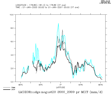
LMDZORnudge.nogustZ0_2000_2009_mix
