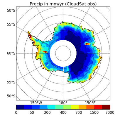
precipSH-OBS
