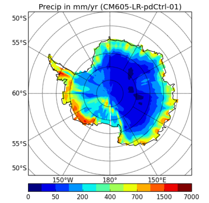
precipSH-CM605-LR-pdCtrl-01
