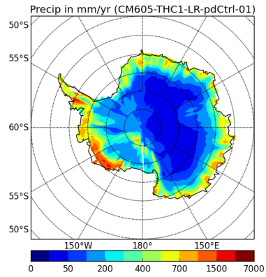
precipSH-CM605-THC1-LR-pdCtrl-01
