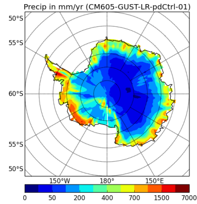
precipSH-CM605-GUST-LR-pdCtrl-01
