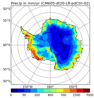
precipSH-CM605-dt20-LR-pdCtrl-02
