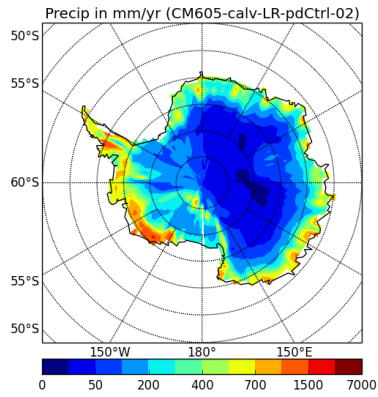
precipSH-CM605-calv-LR-pdCtrl-02
