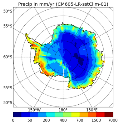
precipSH-CM605-LR-sstClim-01
