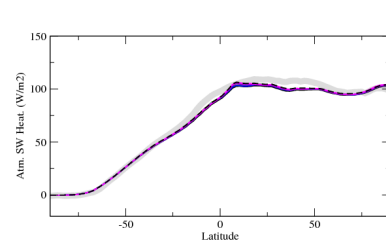
rsahzone
