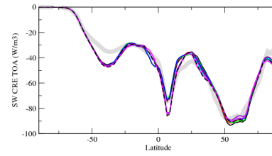
crestzon
