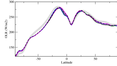
rlutzone
