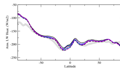
rlahzone
