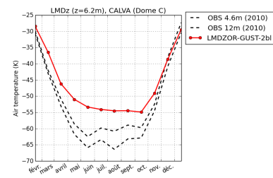
tempDC-LMDZOR-GUST-2bl
