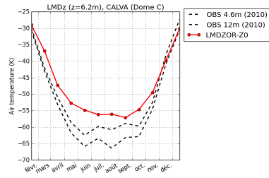
tempDC-LMDZOR-Z0
