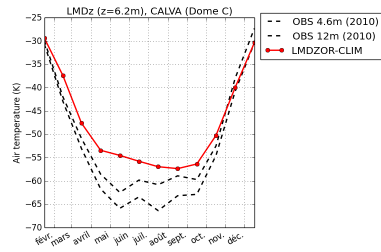
tempDC-LMDZOR-CLIM
