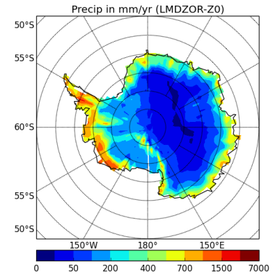
precipSH-LMDZOR-Z0
