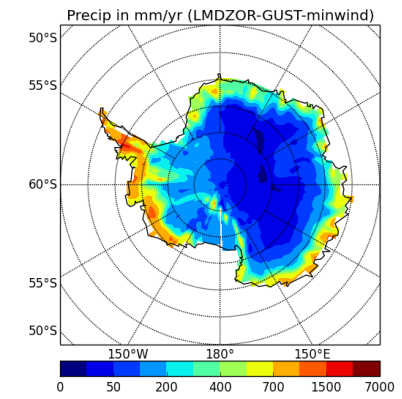
precipSH-LMDZOR-GUST-minwind
