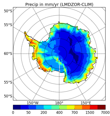
precipSH-LMDZOR-CLIM
