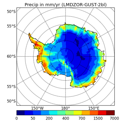
precipSH-LMDZOR-GUST-2bl
