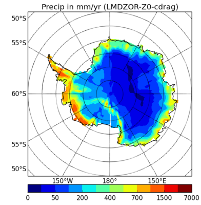
precipSH-LMDZOR-Z0-cdrag
