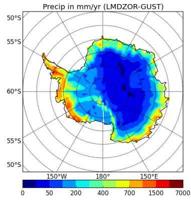
precipSH-LMDZOR-GUST
