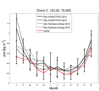
prw_DC_LMDZ.8OMP_1980_1980
