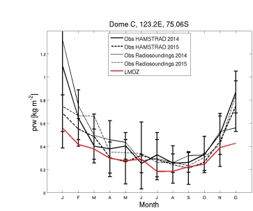
prw_DC_LMDZ.12OMP_1980_1980
