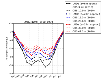
tempDC-LMDZ-8OMP_1980_1980
