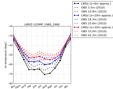
tempDC-LMDZ-12OMP_1980_1980
