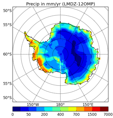
precipSH-LMDZ-12OMP
