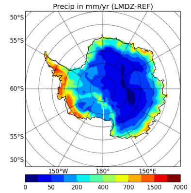
precipSH-LMDZ-REF
