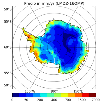
precipSH-LMDZ-16OMP
