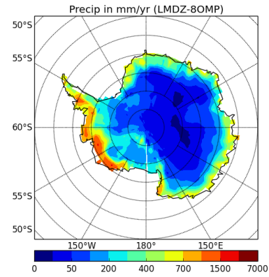
precipSH-LMDZ-8OMP
