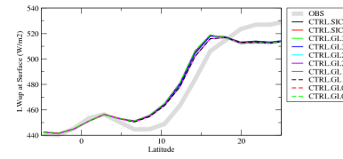
rlusazon
