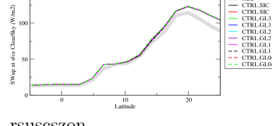
rsuscsazon
