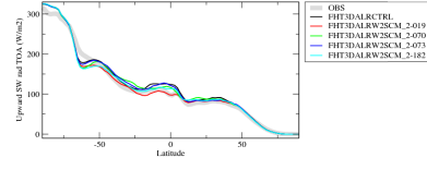
rsutazon
