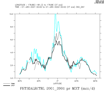
FHT3DALRCTRL_2001_2001_mix
