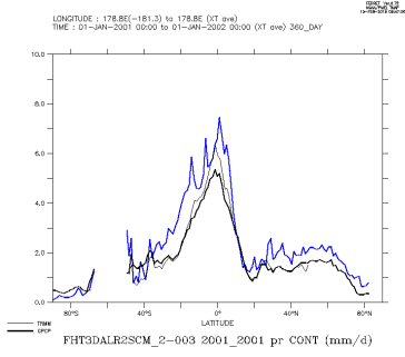
FHT3DALR2SCM_2-003_2001_2001_con
