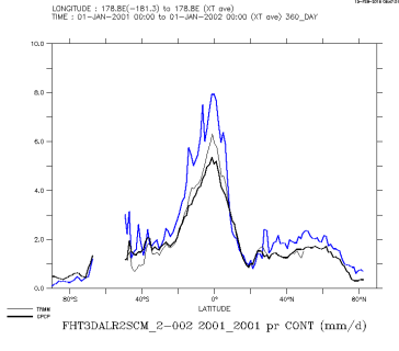
FHT3DALR2SCM_2-002_2001_2001_con
