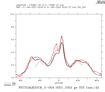
FHT3DALR2SCM_2-004_2001_2001_tot
