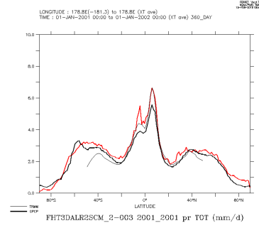
FHT3DALR2SCM_2-003_2001_2001_tot
