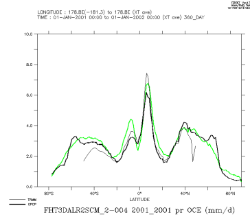
FHT3DALR2SCM_2-004_2001_2001_oce
