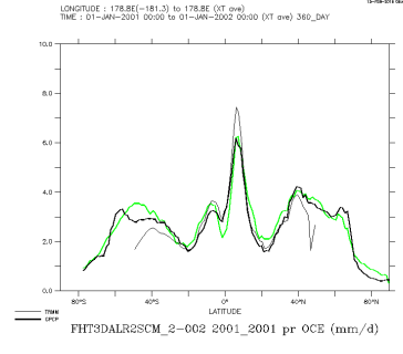
FHT3DALR2SCM_2-002_2001_2001_oce
