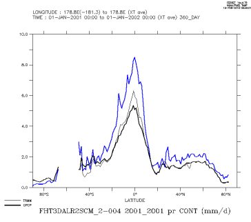
FHT3DALR2SCM_2-004_2001_2001_con
