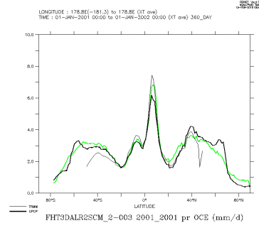
FHT3DALR2SCM_2-003_2001_2001_oce
