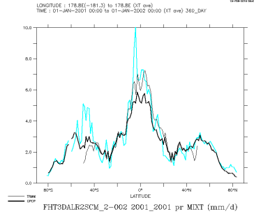
FHT3DALR2SCM_2-002_2001_2001_mix
