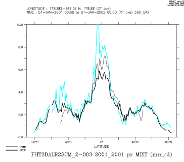
FHT3DALR2SCM_2-003_2001_2001_mix
