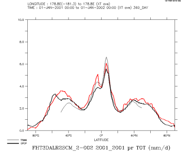
FHT3DALR2SCM_2-002_2001_2001_tot
