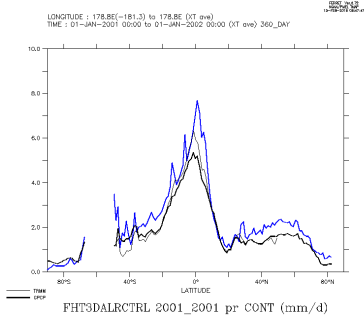
FHT3DALRCTRL_2001_2001_con
