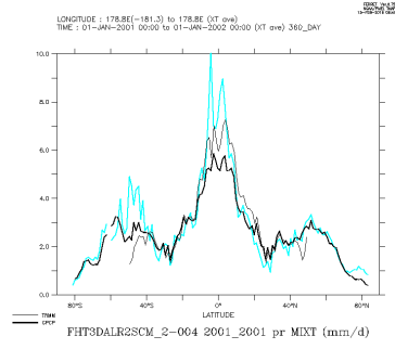
FHT3DALR2SCM_2-004_2001_2001_mix
