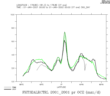
FHT3DALRCTRL_2001_2001_oce
